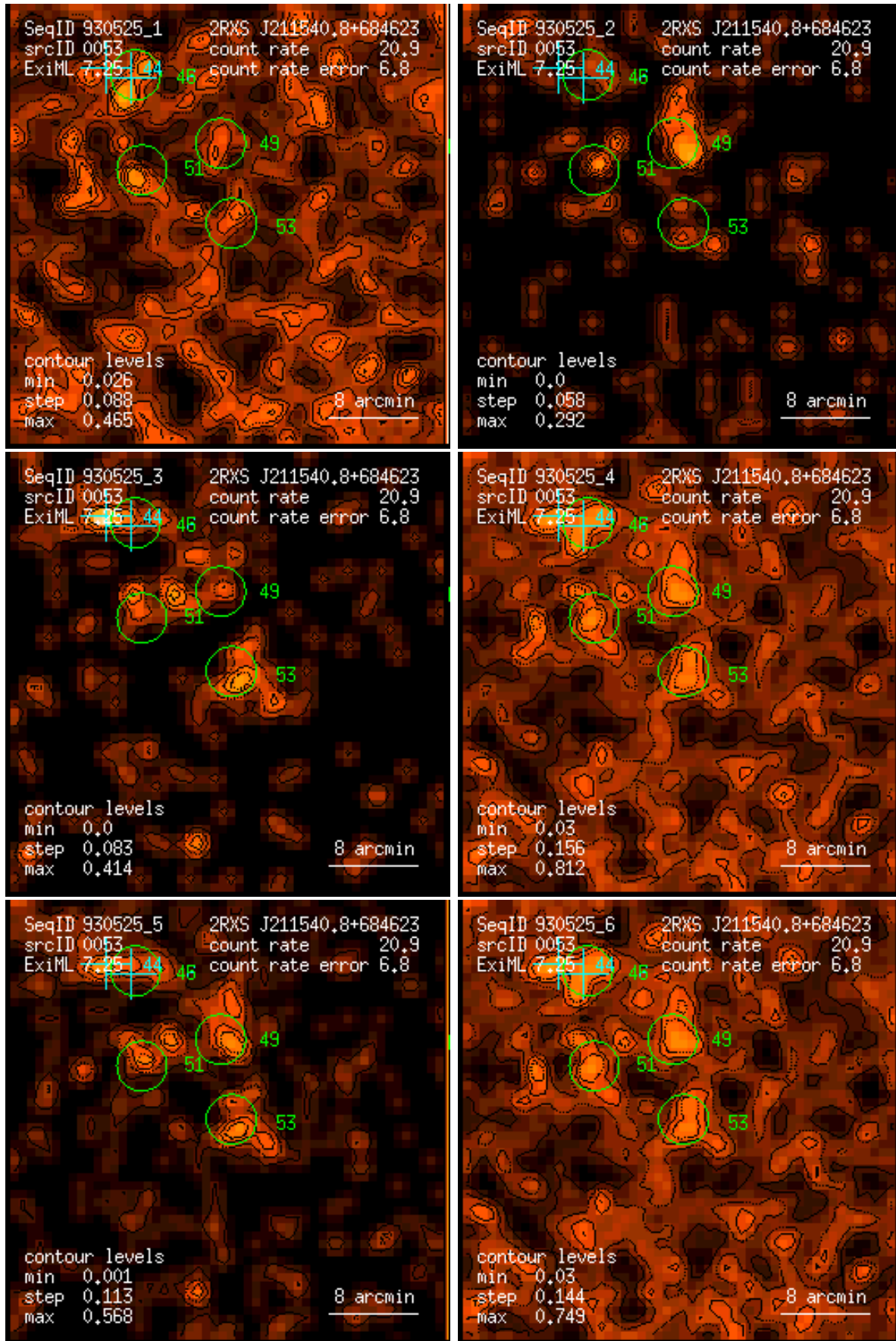
Figure 53: RASS 930525: detection 0053: band rate images, Gaussian filter: (1) PSPC channels 11 – 41, (2) 52 – 90, (3) 91 – 201, (4) 11 – 235, (5) 52 – 201, (6) 11 – 201. Broad band rates in counts/ks. Band rate contour levels in counts/ks/arcmin 2 .
