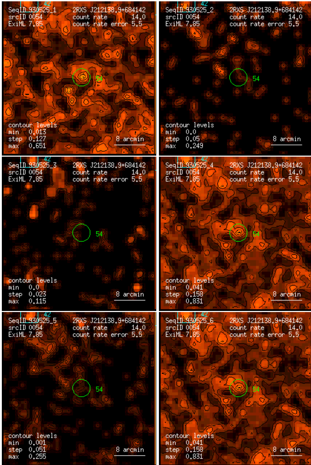
Figure 54: RASS 930525: detection 0054: band rate images, Gaussian filter: (1) PSPC channels 11 – 41, (2) 52 – 90, (3) 91 – 201, (4) 11 – 235, (5) 52 – 201, (6) 11 – 201. Broad band rates in counts/ks. Band rate contour levels in counts/ks/arcmin 2 .
