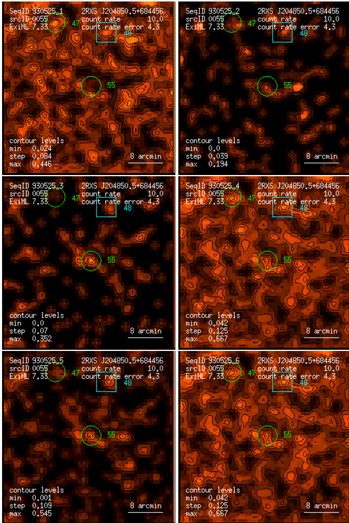
Figure 55: RASS 930525: detection 0055: band rate images, Gaussian filter: (1) PSPC channels 11 – 41, (2) 52 – 90, (3) 91 – 201, (4) 11 – 235, (5) 52 – 201, (6) 11 – 201. Broad band rates in counts/ks. Band rate contour levels in counts/ks/arcmin 2 .
