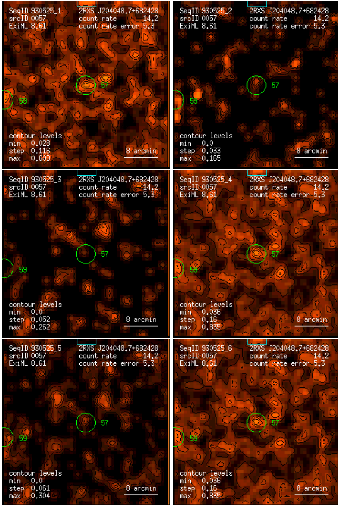
Figure 57: RASS 930525: detection 0057: band rate images, Gaussian filter: (1) PSPC channels 11 – 41, (2) 52 – 90, (3) 91 – 201, (4) 11 – 235, (5) 52 – 201, (6) 11 – 201. Broad band rates in counts/ks. Band rate contour levels in counts/ks/arcmin 2 .
