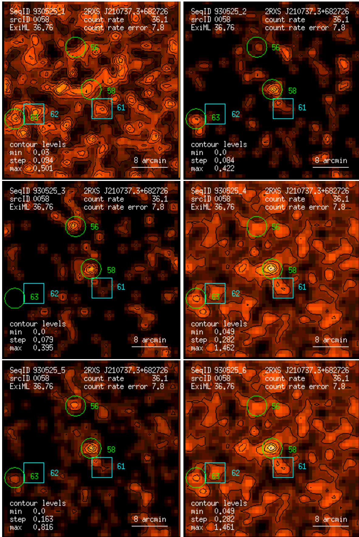
Figure 58: RASS 930525: detection 0058: band rate images, Gaussian filter: (1) PSPC channels 11 – 41, (2) 52 – 90, (3) 91 – 201, (4) 11 – 235, (5) 52 – 201, (6) 11 – 201. Broad band rates in counts/ks. Band rate contour levels in counts/ks/arcmin 2 .
