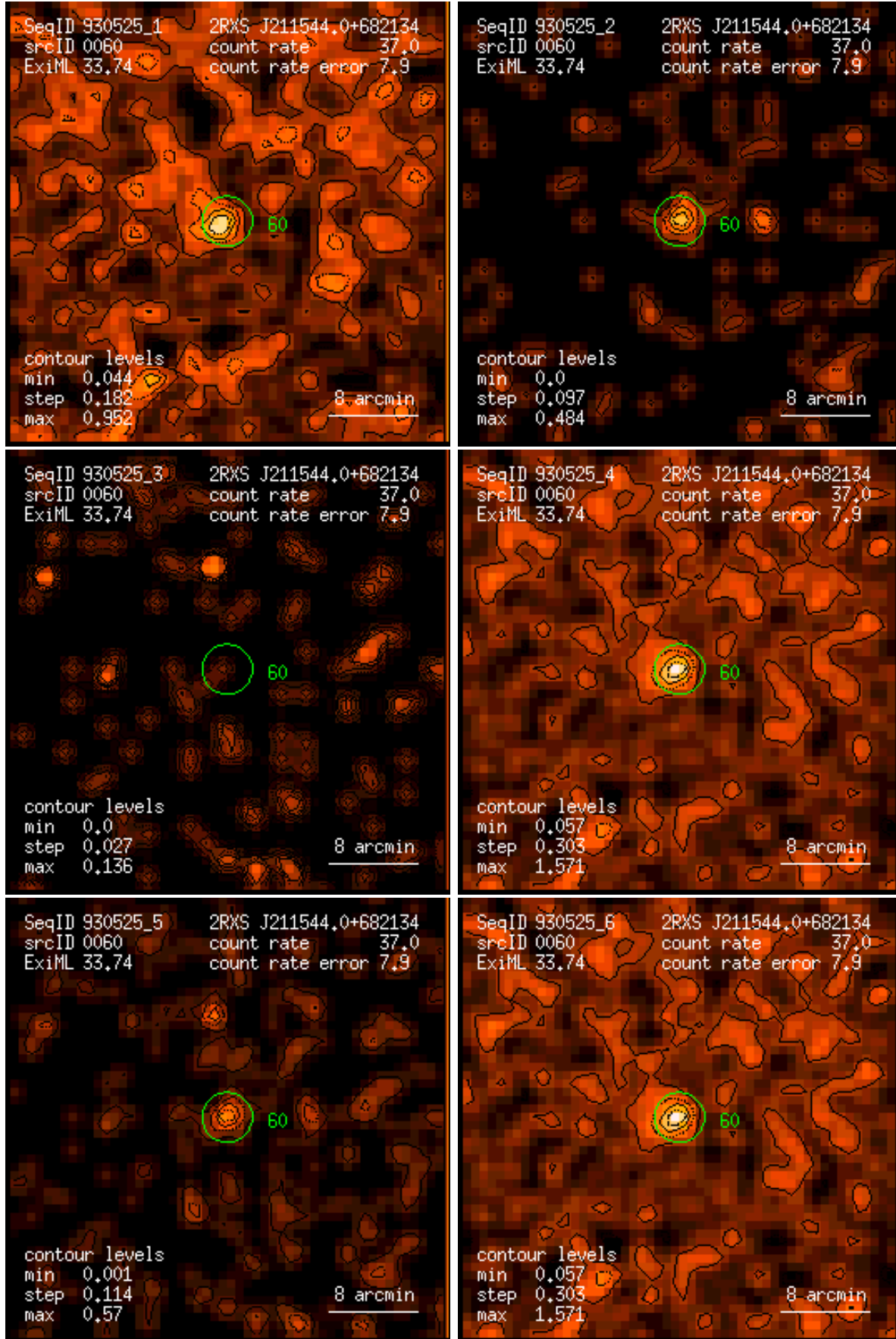
Figure 60: RASS 930525: detection 0060: band rate images, Gaussian filter: (1) PSPC channels 11 – 41, (2) 52 – 90, (3) 91 – 201, (4) 11 – 235, (5) 52 – 201, (6) 11 – 201. Broad band rates in counts/ks. Band rate contour levels in counts/ks/arcmin 2 .
