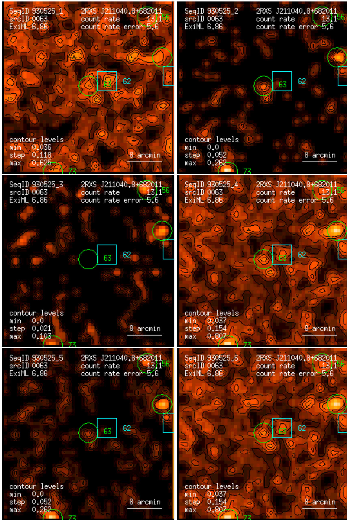
Figure 63: RASS 930525: detection 0063: band rate images, Gaussian filter: (1) PSPC channels 11 – 41, (2) 52 – 90, (3) 91 – 201, (4) 11 – 235, (5) 52 – 201, (6) 11 – 201. Broad band rates in counts/ks. Band rate contour levels in counts/ks/arcmin 2 .
