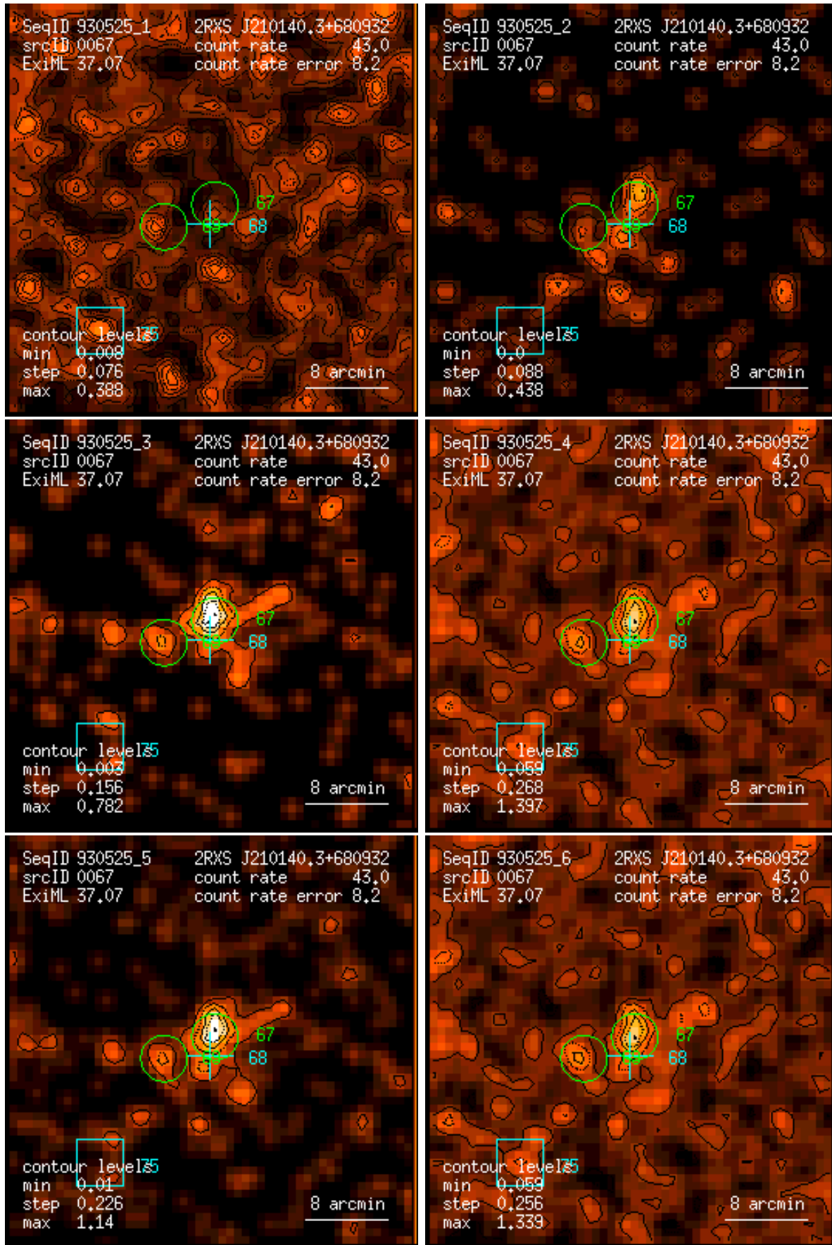
Figure 67: RASS 930525: detection 0067: band rate images, Gaussian filter: (1) PSPC channels 11 – 41, (2) 52 – 90, (3) 91 – 201, (4) 11 – 235, (5) 52 – 201, (6) 11 – 201. Broad band rates in counts/ks. Band rate contour levels in counts/ks/arcmin 2 .
