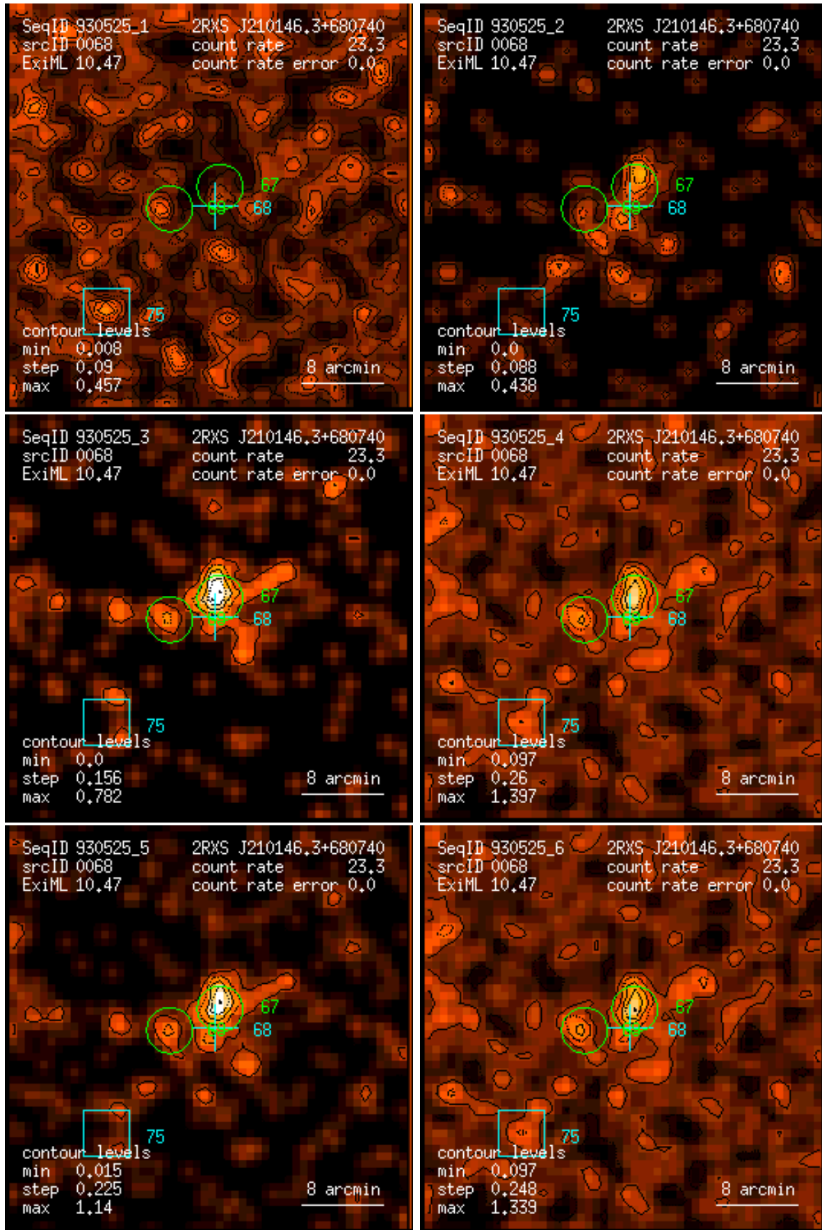
Figure 68: RASS 930525: detection 0068: band rate images, Gaussian filter: (1) PSPC channels 11 – 41, (2) 52 – 90, (3) 91 – 201, (4) 11 – 235, (5) 52 – 201, (6) 11 – 201. Broad band rates in counts/ks. Band rate contour levels in counts/ks/arcmin 2 .
