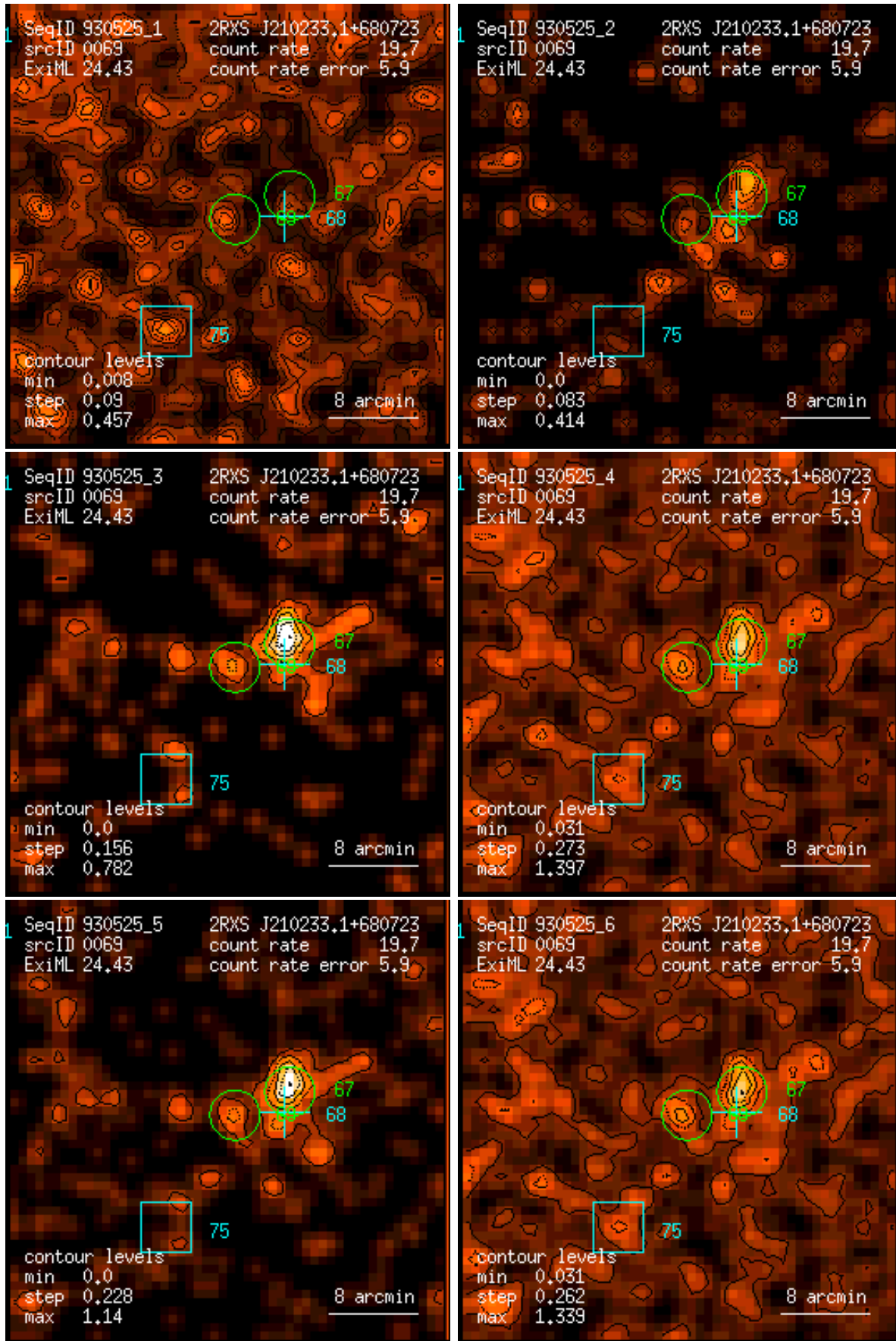
Figure 69: RASS 930525: detection 0069: band rate images, Gaussian filter: (1) PSPC channels 11 – 41, (2) 52 – 90, (3) 91 – 201, (4) 11 – 235, (5) 52 – 201, (6) 11 – 201. Broad band rates in counts/ks. Band rate contour levels in counts/ks/arcmin 2 .
