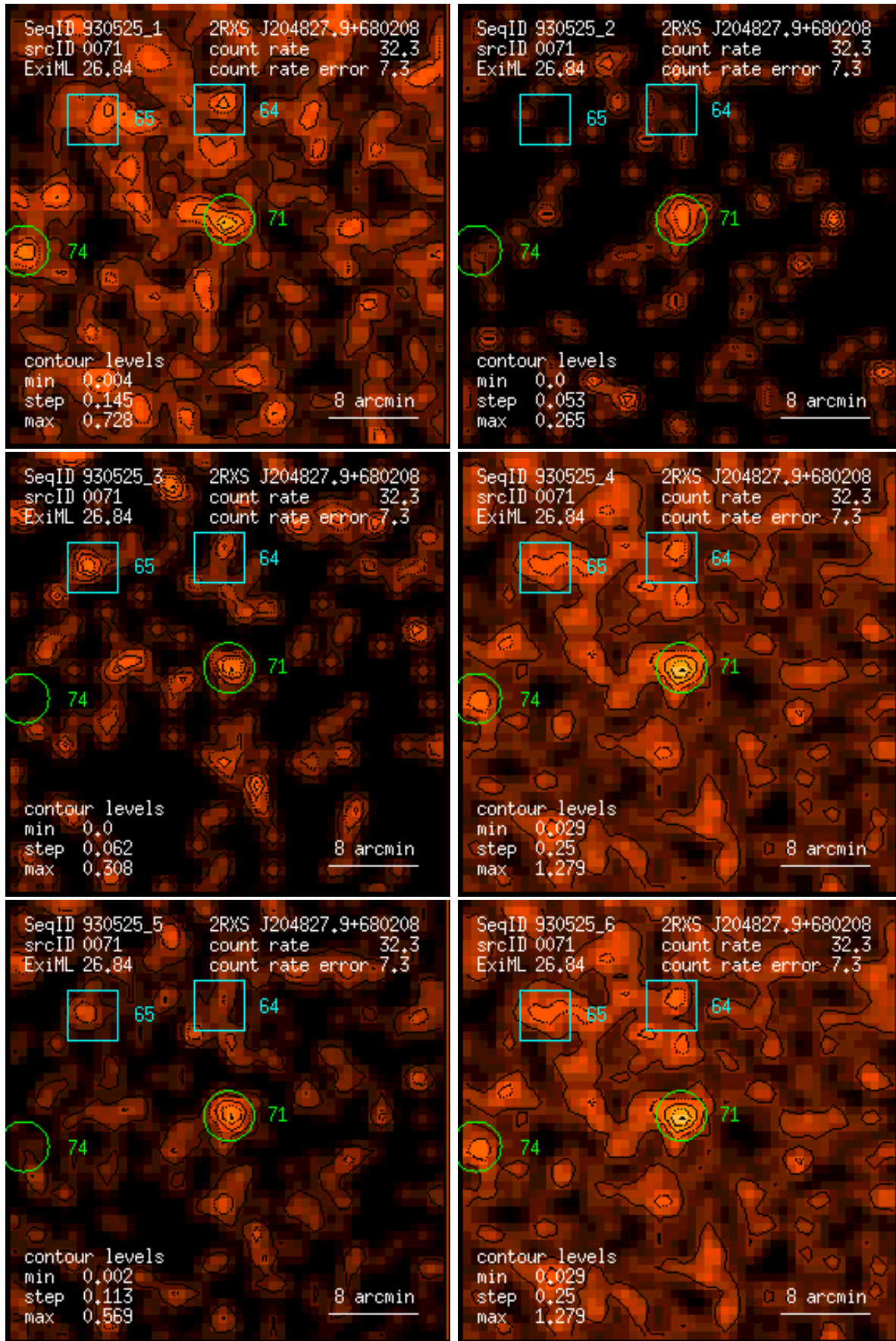
Figure 71: RASS 930525: detection 0071: band rate images, Gaussian filter: (1) PSPC channels 11 – 41, (2) 52 – 90, (3) 91 – 201, (4) 11 – 235, (5) 52 – 201, (6) 11 – 201. Broad band rates in counts/ks. Band rate contour levels in counts/ks/arcmin 2 .
