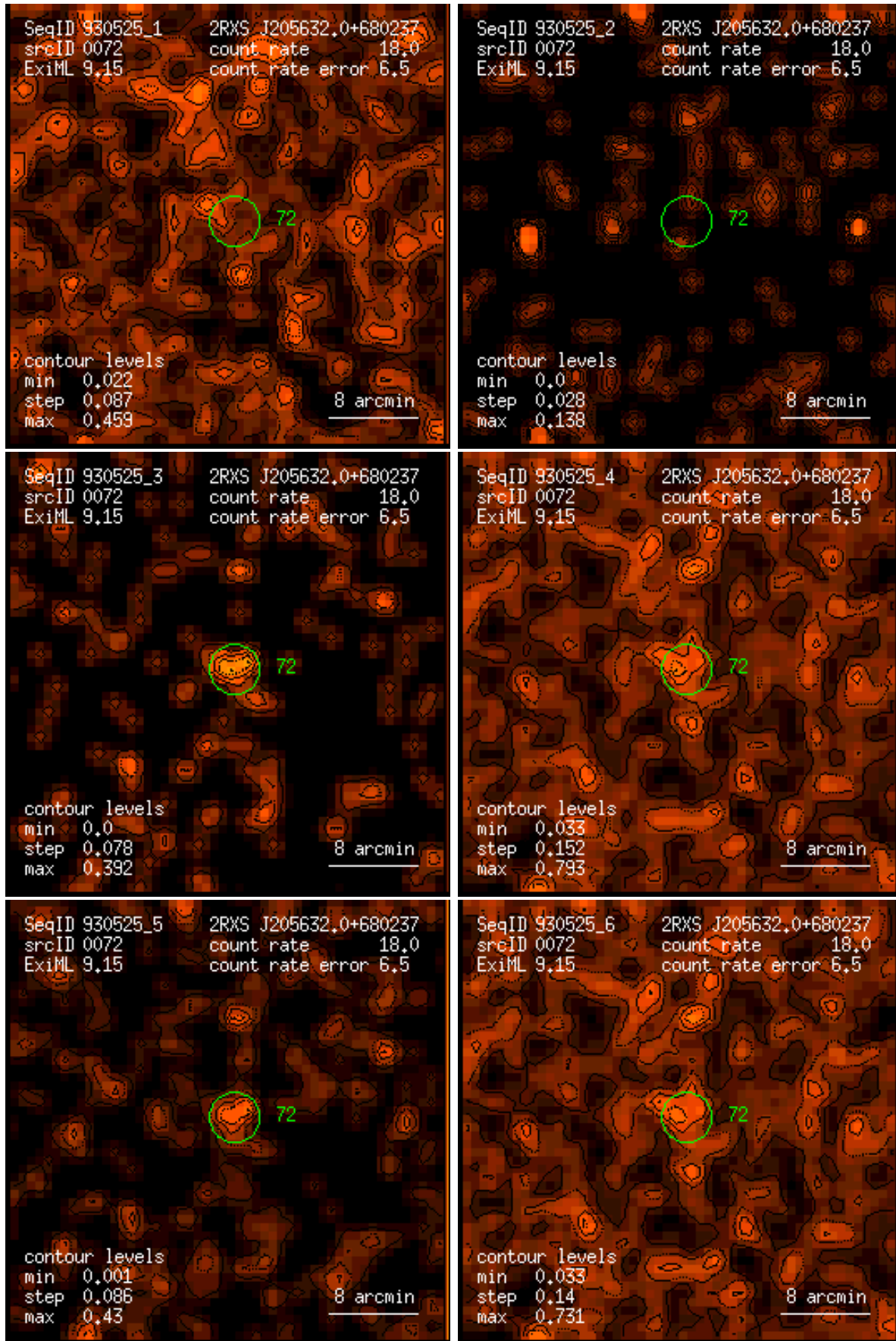
Figure 72: RASS 930525: detection 0072: band rate images, Gaussian filter: (1) PSPC channels 11 – 41, (2) 52 – 90, (3) 91 – 201, (4) 11 – 235, (5) 52 – 201, (6) 11 – 201. Broad band rates in counts/ks. Band rate contour levels in counts/ks/arcmin 2 .
