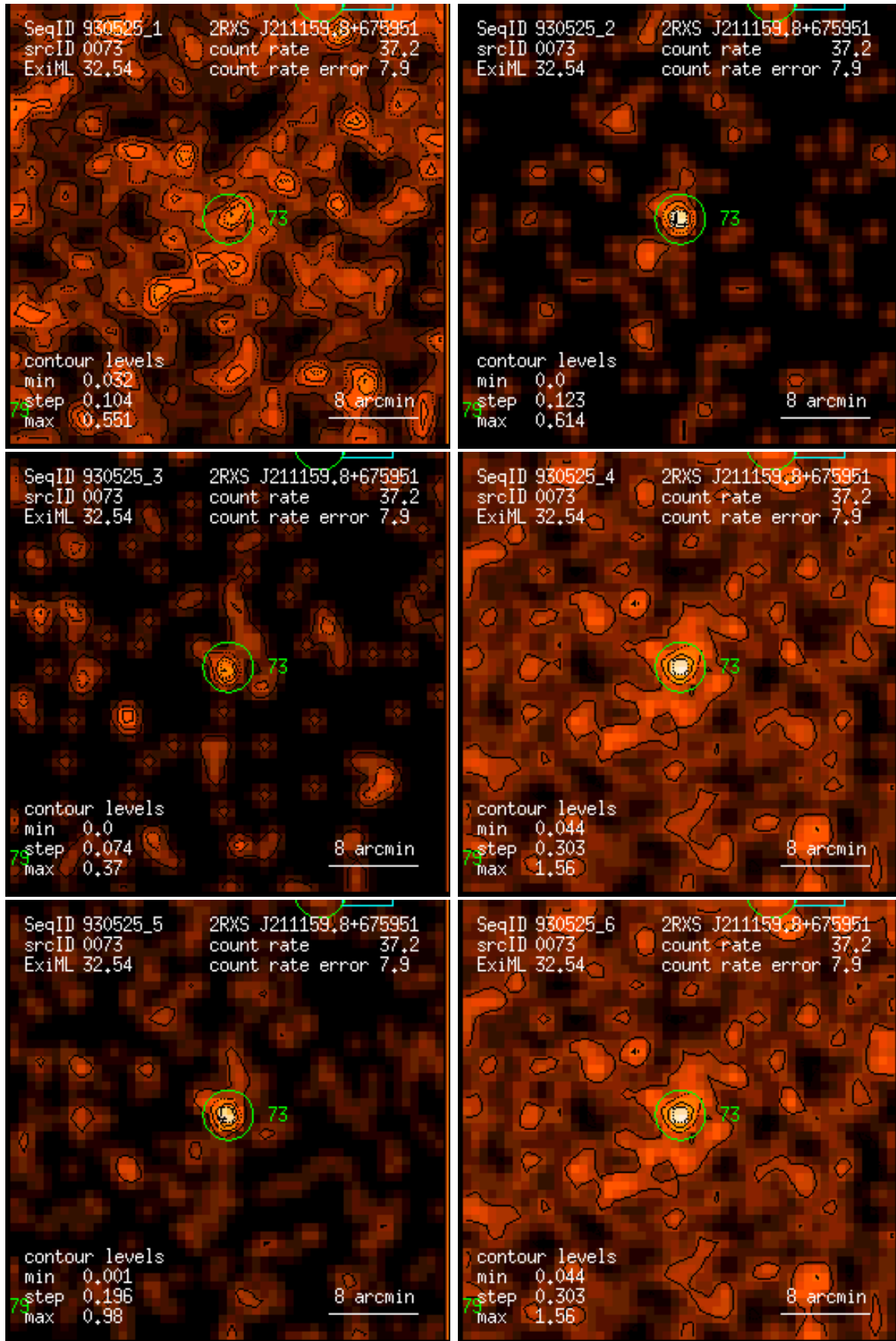
Figure 73: RASS 930525: detection 0073: band rate images, Gaussian filter: (1) PSPC channels 11 – 41, (2) 52 – 90, (3) 91 – 201, (4) 11 – 235, (5) 52 – 201, (6) 11 – 201. Broad band rates in counts/ks. Band rate contour levels in counts/ks/arcmin 2 .
