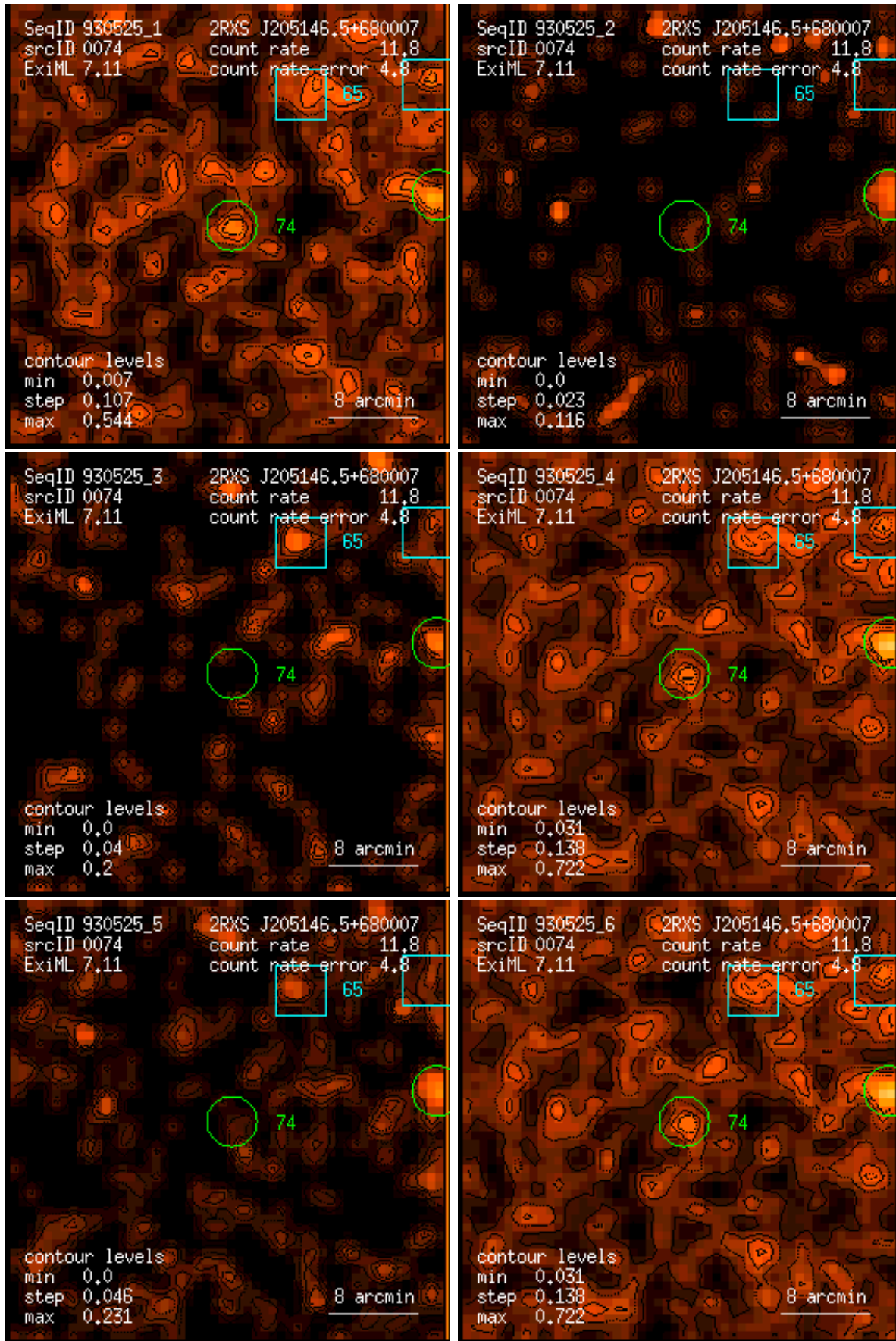
Figure 74: RASS 930525: detection 0074: band rate images, Gaussian filter: (1) PSPC channels 11 – 41, (2) 52 – 90, (3) 91 – 201, (4) 11 – 235, (5) 52 – 201, (6) 11 – 201. Broad band rates in counts/ks. Band rate contour levels in counts/ks/arcmin 2 .
