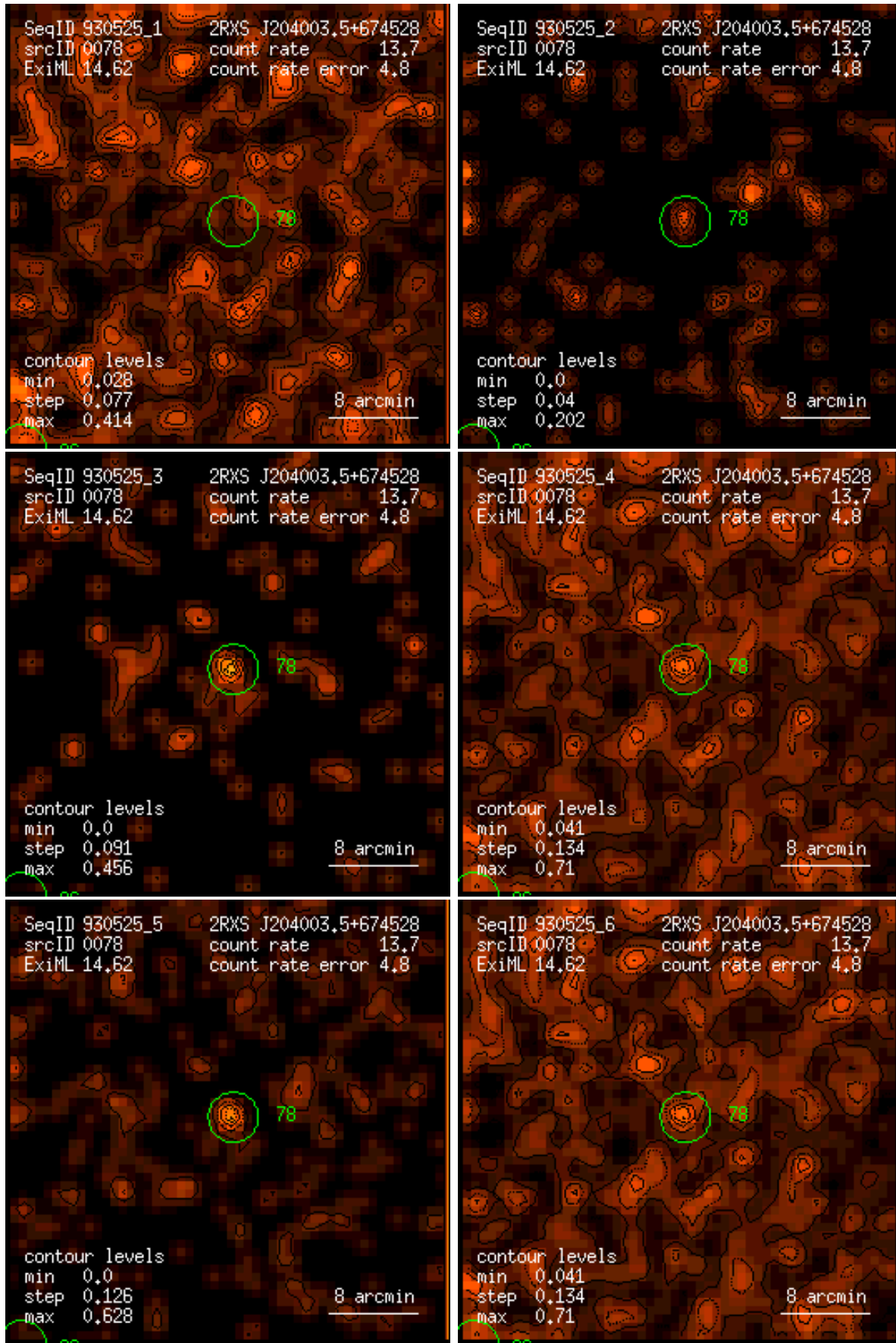
Figure 78: RASS 930525: detection 0078: band rate images, Gaussian filter: (1) PSPC channels 11 – 41, (2) 52 – 90, (3) 91 – 201, (4) 11 – 235, (5) 52 – 201, (6) 11 – 201. Broad band rates in counts/ks. Band rate contour levels in counts/ks/arcmin 2 .
