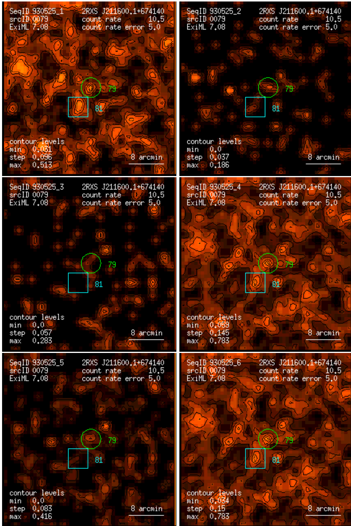
Figure 79: RASS 930525: detection 0079: band rate images, Gaussian filter: (1) PSPC channels 11 – 41, (2) 52 – 90, (3) 91 – 201, (4) 11 – 235, (5) 52 – 201, (6) 11 – 201. Broad band rates in counts/ks. Band rate contour levels in counts/ks/arcmin 2 .
