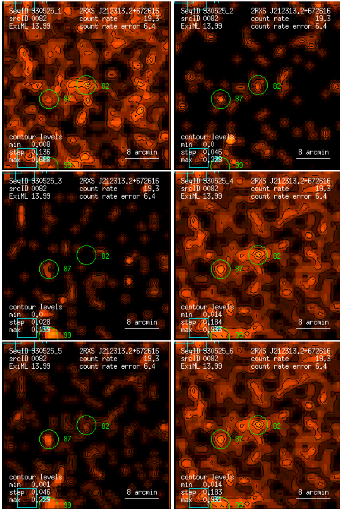
Figure 82: RASS 930525: detection 0082: band rate images, Gaussian filter: (1) PSPC channels 11 – 41, (2) 52 – 90, (3) 91 – 201, (4) 11 – 235, (5) 52 – 201, (6) 11 – 201. Broad band rates in counts/ks. Band rate contour levels in counts/ks/arcmin 2 .
