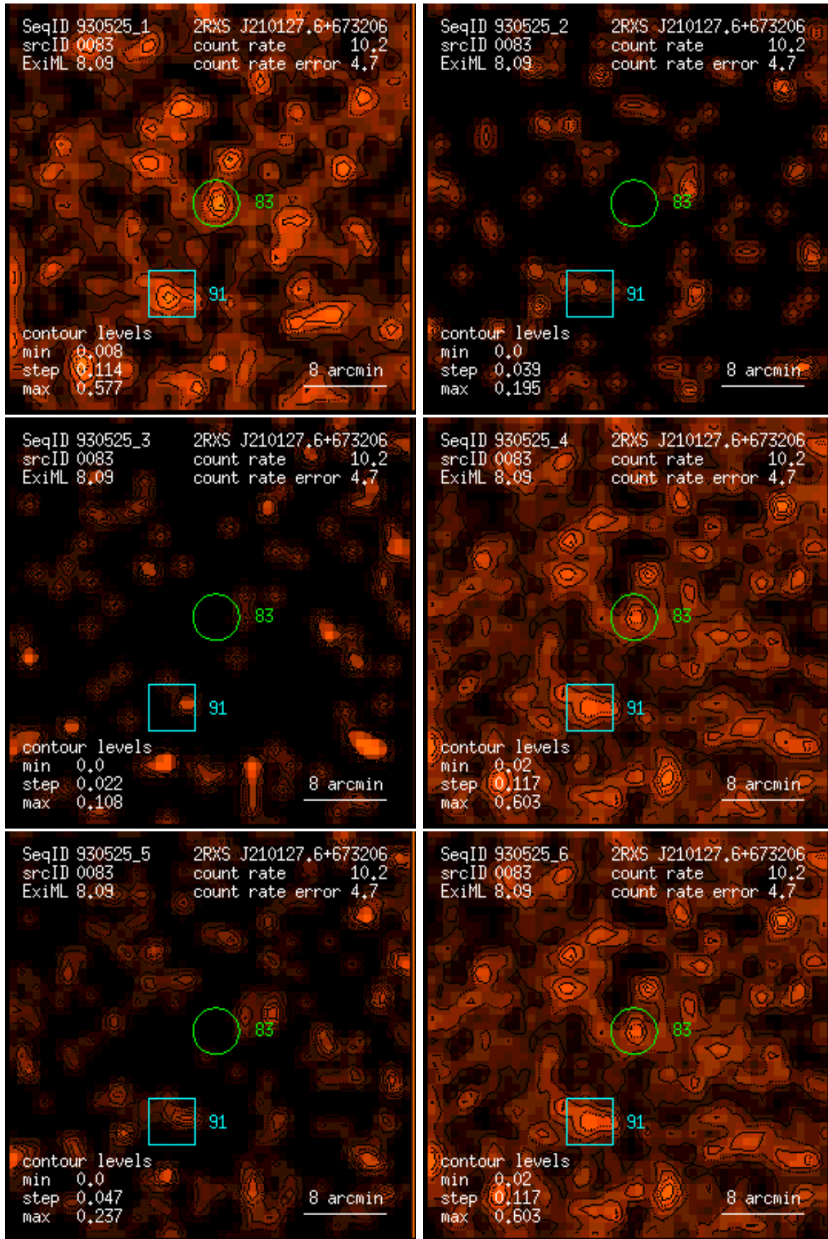
Figure 83: RASS 930525: detection 0083: band rate images, Gaussian filter: (1) PSPC channels 11 – 41, (2) 52 – 90, (3) 91 – 201, (4) 11 – 235, (5) 52 – 201, (6) 11 – 201. Broad band rates in counts/ks. Band rate contour levels in counts/ks/arcmin 2 .
