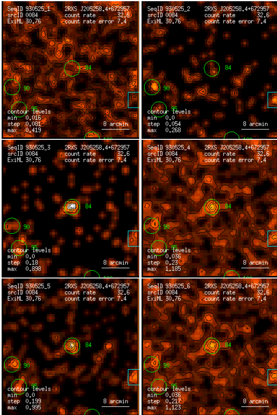
Figure 84: RASS 930525: detection 0084: band rate images, Gaussian filter: (1) PSPC channels 11 – 41, (2) 52 – 90, (3) 91 – 201, (4) 11 – 235, (5) 52 – 201, (6) 11 – 201. Broad band rates in counts/ks. Band rate contour levels in counts/ks/arcmin 2 .
