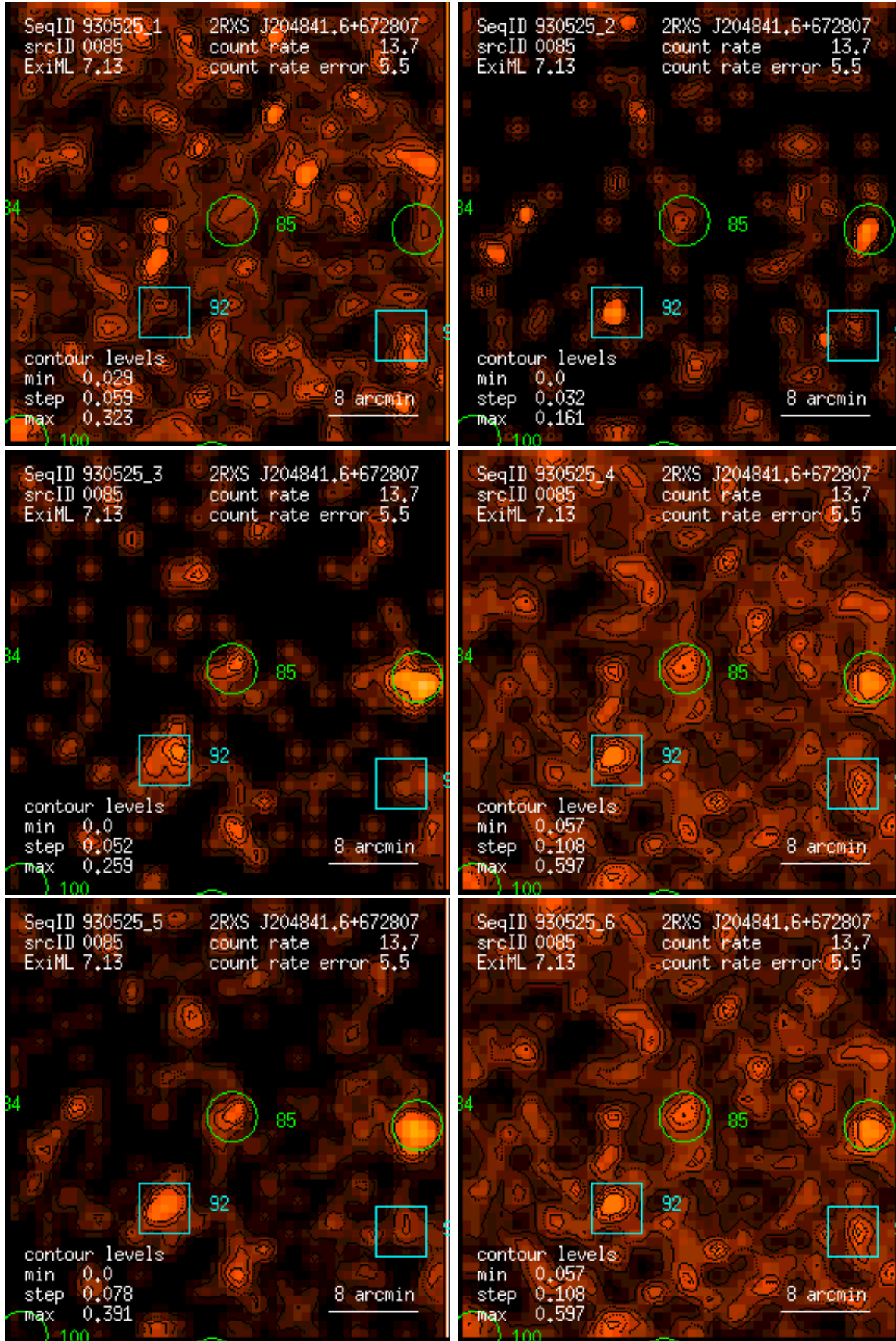
Figure 85: RASS 930525: detection 0085: band rate images, Gaussian filter: (1) PSPC channels 11 – 41, (2) 52 – 90, (3) 91 – 201, (4) 11 – 235, (5) 52 – 201, (6) 11 – 201. Broad band rates in counts/ks. Band rate contour levels in counts/ks/arcmin 2 .
