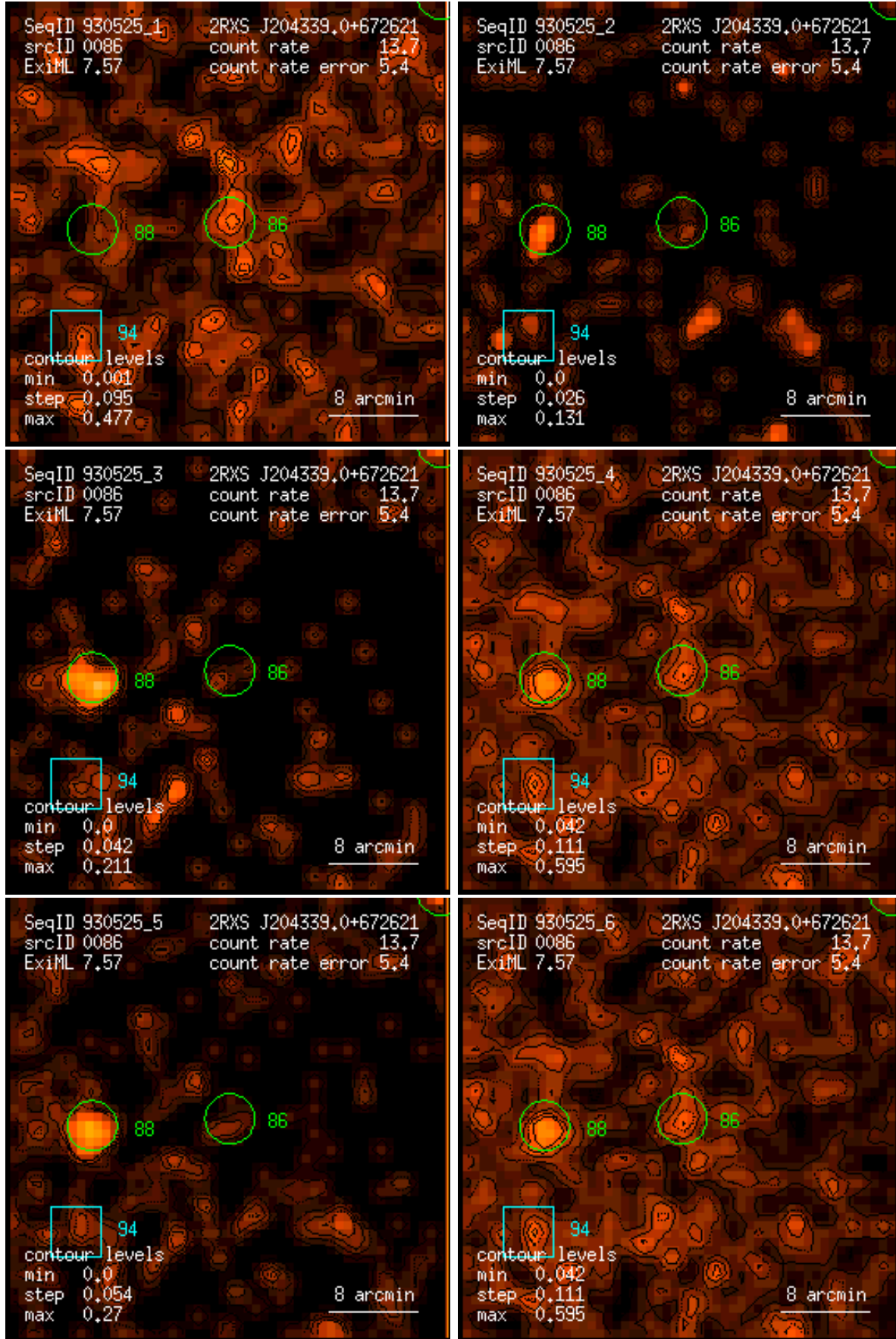
Figure 86: RASS 930525: detection 0086: band rate images, Gaussian filter: (1) PSPC channels 11 – 41, (2) 52 – 90, (3) 91 – 201, (4) 11 – 235, (5) 52 – 201, (6) 11 – 201. Broad band rates in counts/ks. Band rate contour levels in counts/ks/arcmin 2 .
