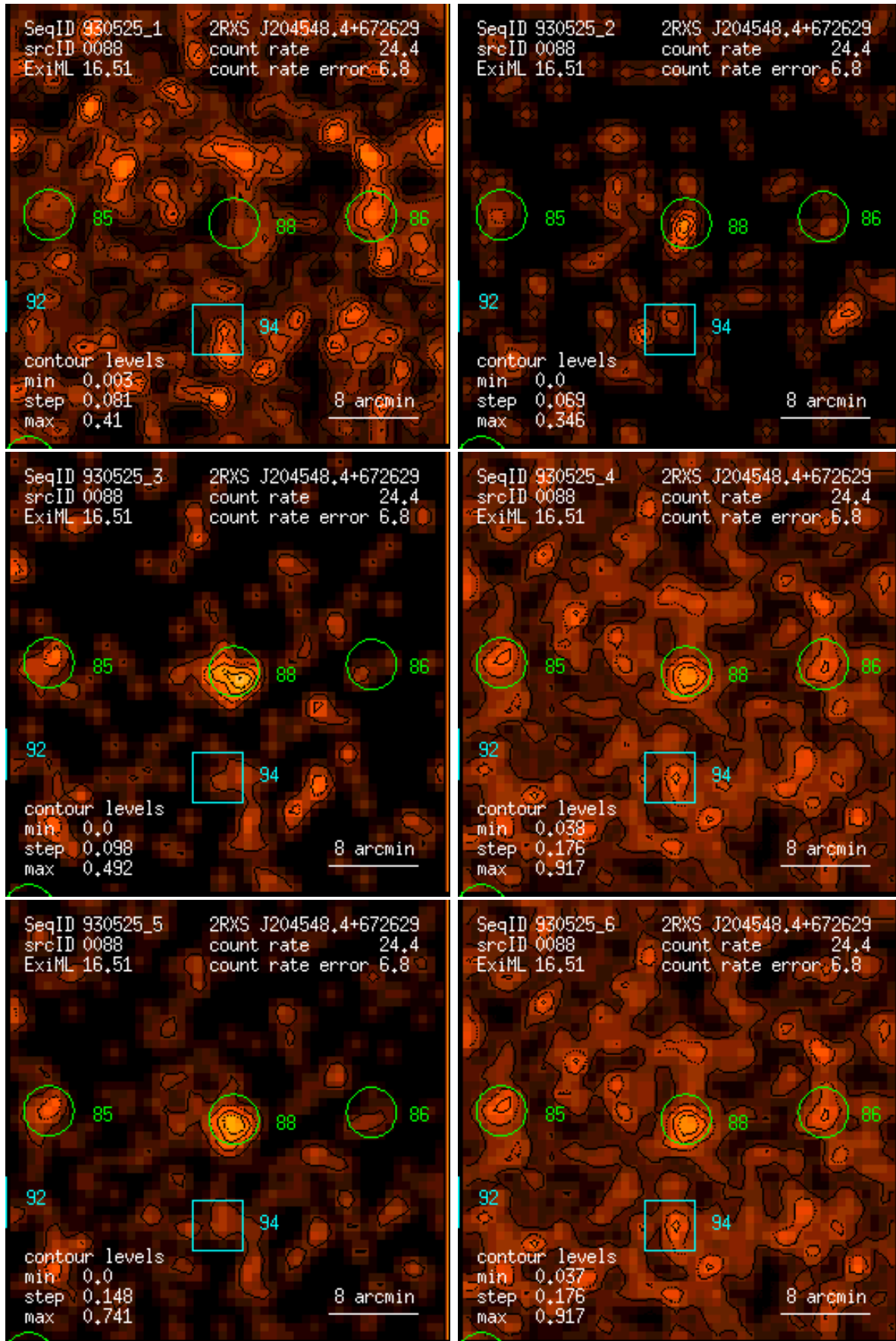
Figure 88: RASS 930525: detection 0088: band rate images, Gaussian filter: (1) PSPC channels 11 – 41, (2) 52 – 90, (3) 91 – 201, (4) 11 – 235, (5) 52 – 201, (6) 11 – 201. Broad band rates in counts/ks. Band rate contour levels in counts/ks/arcmin 2 .
