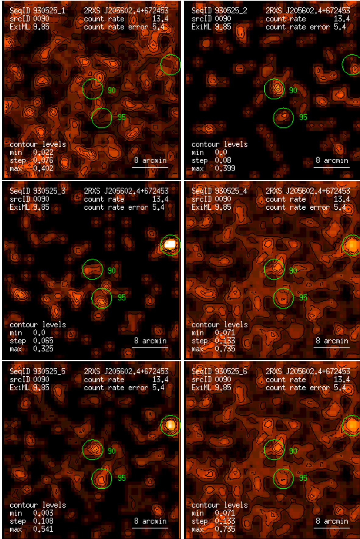
Figure 90: RASS 930525: detection 0090: band rate images, Gaussian filter: (1) PSPC channels 11 – 41, (2) 52 – 90, (3) 91 – 201, (4) 11 – 235, (5) 52 – 201, (6) 11 – 201. Broad band rates in counts/ks. Band rate contour levels in counts/ks/arcmin 2 .
