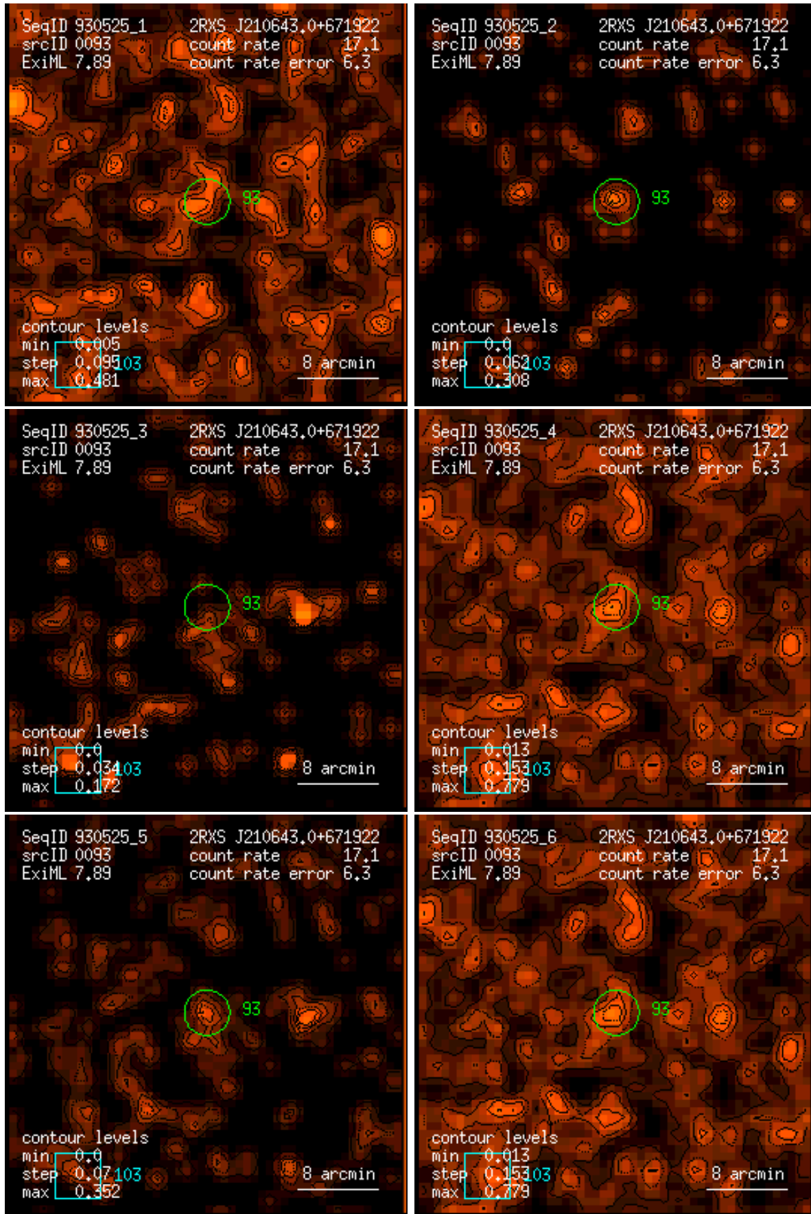
Figure 93: RASS 930525: detection 0093: band rate images, Gaussian filter: (1) PSPC channels 11 – 41, (2) 52 – 90, (3) 91 – 201, (4) 11 – 235, (5) 52 – 201, (6) 11 – 201. Broad band rates in counts/ks. Band rate contour levels in counts/ks/arcmin 2 .
