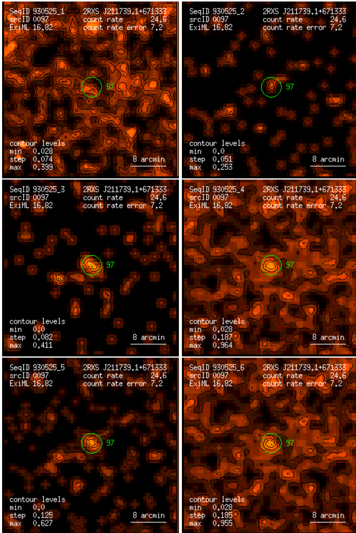
Figure 97: RASS 930525: detection 0097: band rate images, Gaussian filter: (1) PSPC channels 11 – 41, (2) 52 – 90, (3) 91 – 201, (4) 11 – 235, (5) 52 – 201, (6) 11 – 201. Broad band rates in counts/ks. Band rate contour levels in counts/ks/arcmin 2 .
