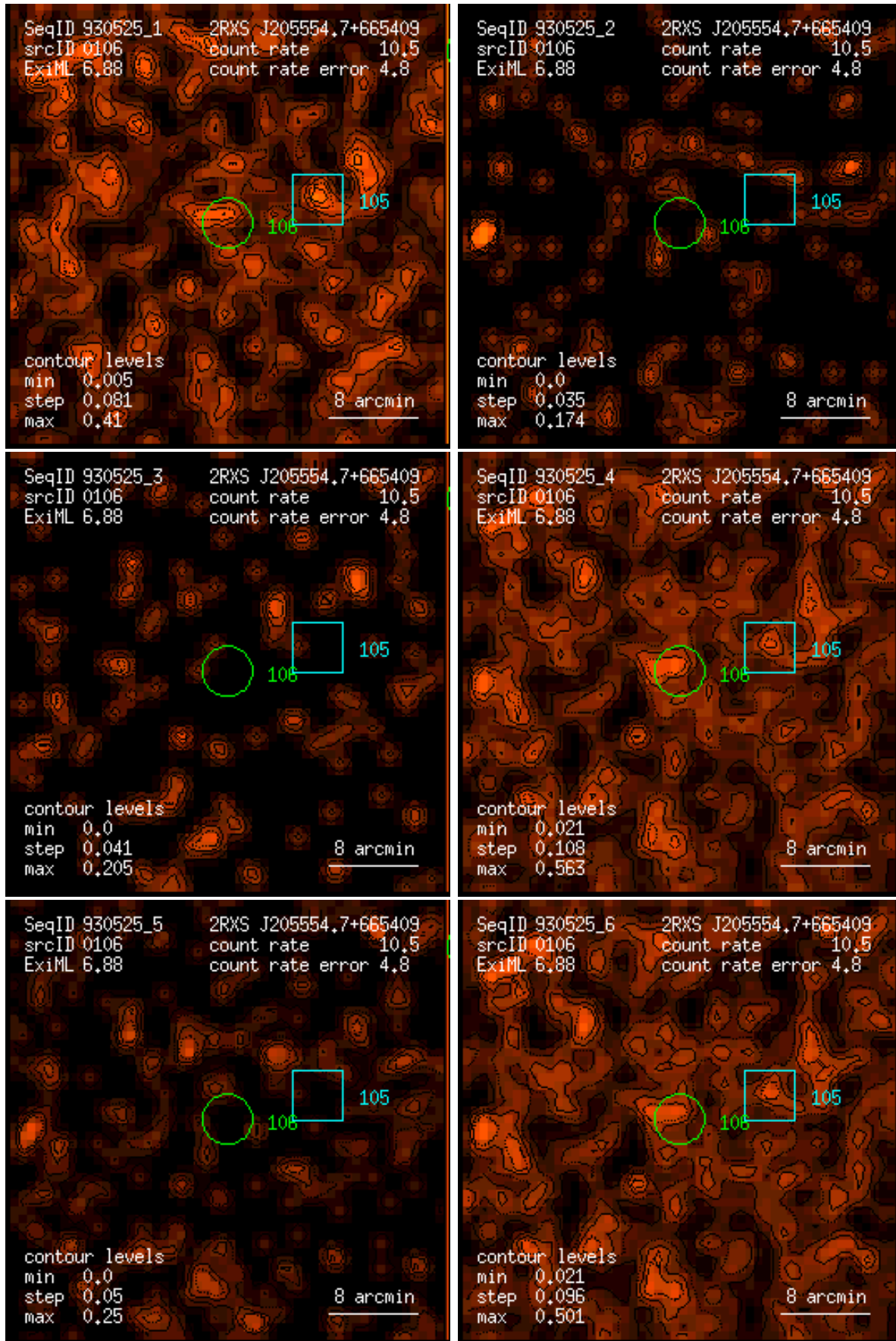
Figure 106: RASS 930525: detection 0106: band rate images, Gaussian filter: (1) PSPC channels 11 – 41, (2) 52 – 90, (3) 91 – 201, (4) 11 – 235, (5) 52 – 201, (6) 11 – 201. Broad band rates in counts/ks. Band rate contour levels in counts/ks/arcmin 2 .
