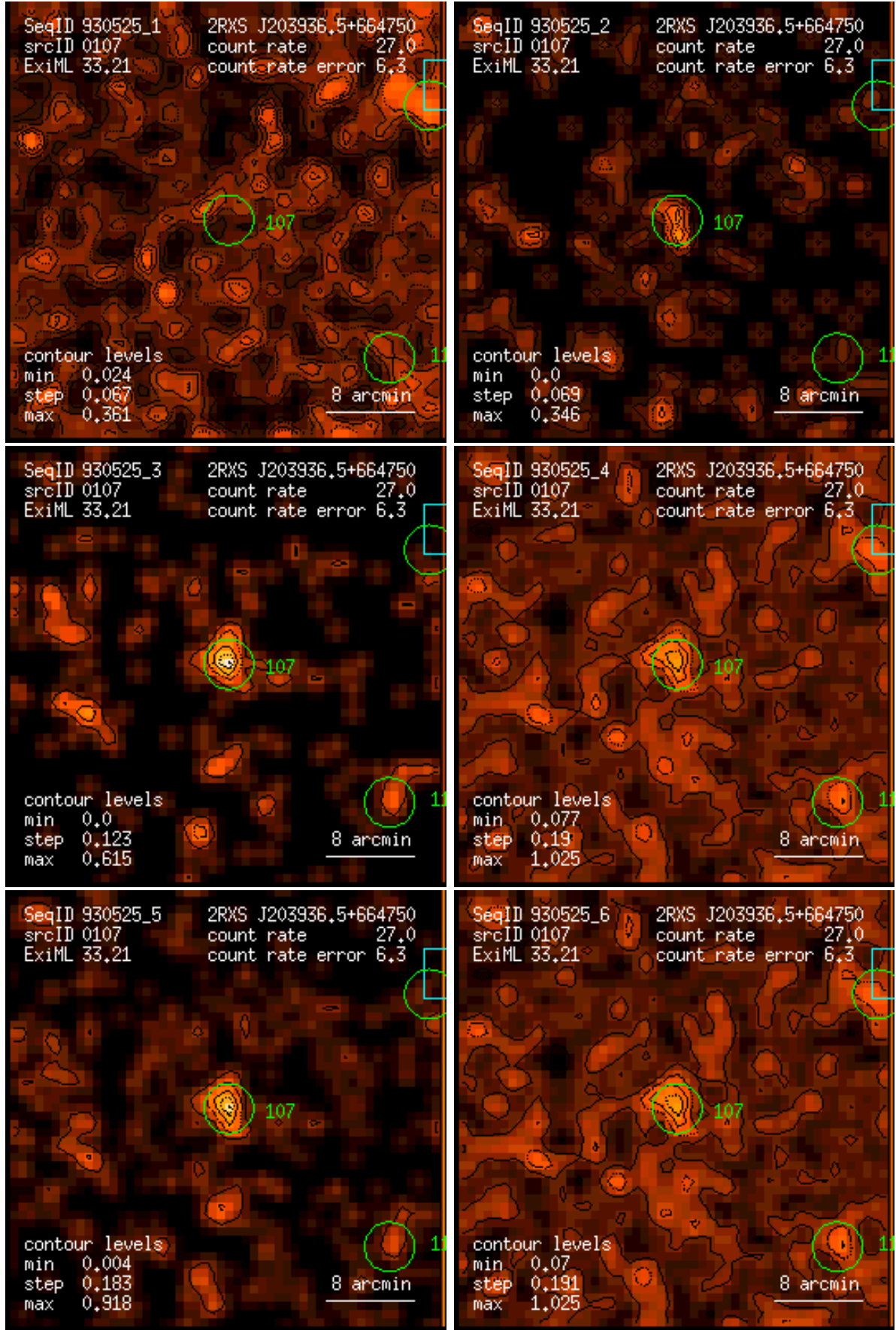
Figure 107: RASS 930525: detection 0107: band rate images, Gaussian filter: (1) PSPC channels 11 – 41, (2) 52 – 90, (3) 91 – 201, (4) 11 – 235, (5) 52 – 201, (6) 11 – 201. Broad band rates in counts/ks. Band rate contour levels in counts/ks/arcmin 2 .
