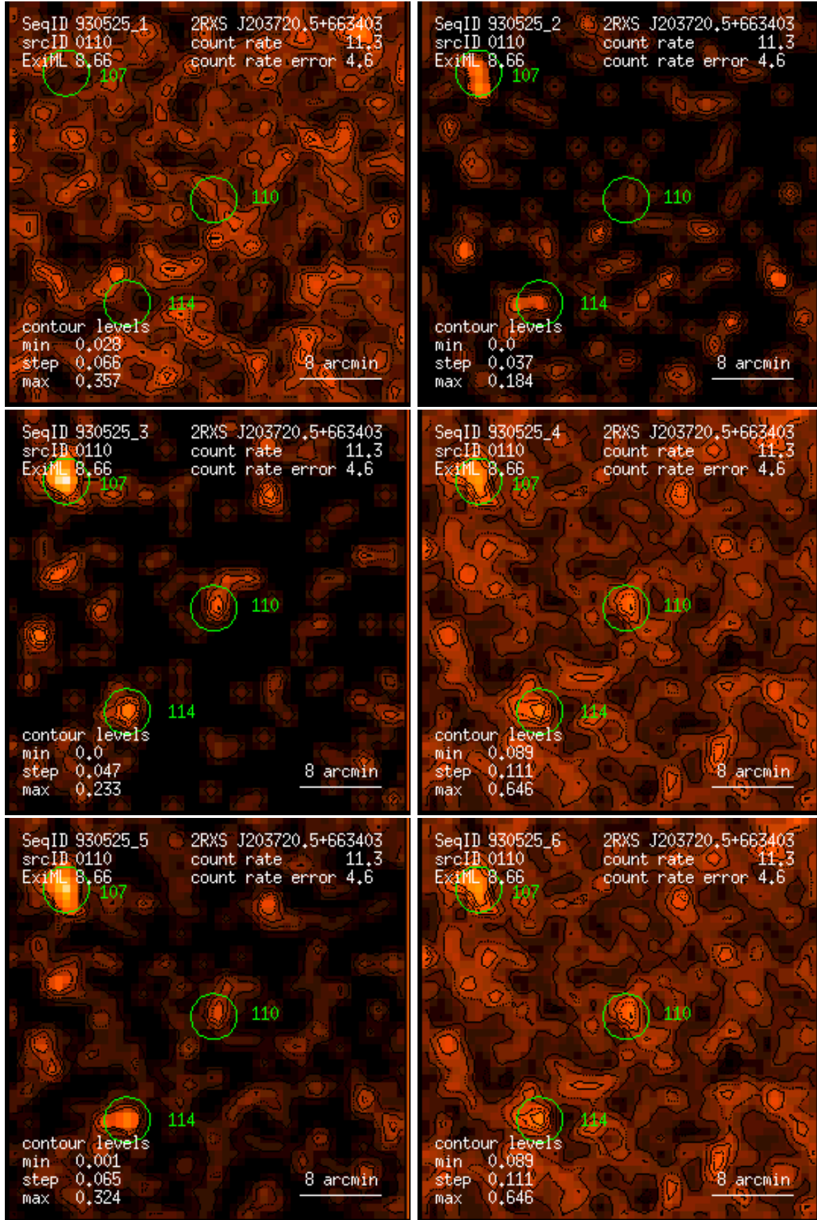
Figure 110: RASS 930525: detection 0110: band rate images, Gaussian filter: (1) PSPC channels 11 – 41, (2) 52 – 90, (3) 91 – 201, (4) 11 – 235, (5) 52 – 201, (6) 11 – 201. Broad band rates in counts/ks. Band rate contour levels in counts/ks/arcmin 2 .
