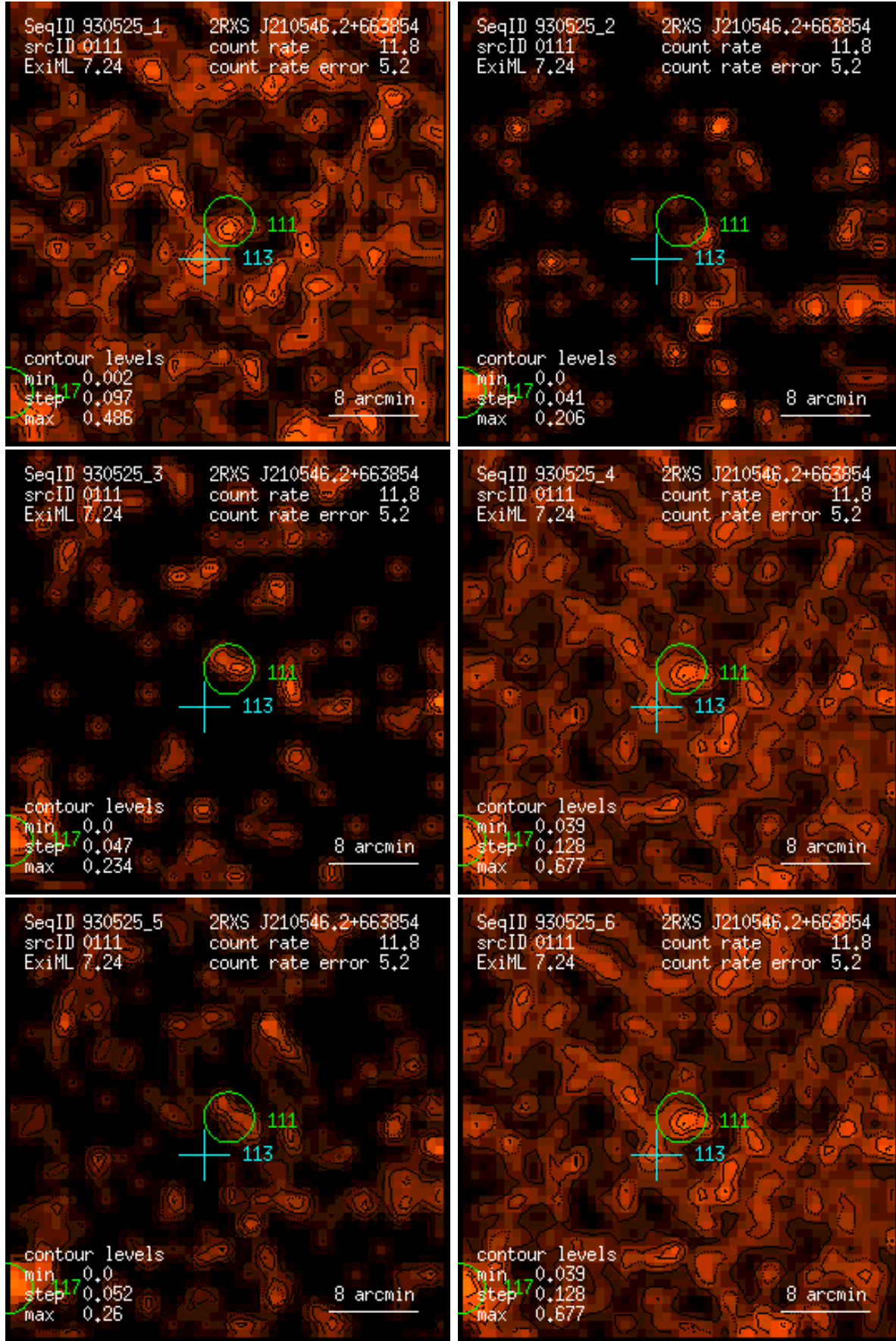
Figure 111: RASS 930525: detection 0111: band rate images, Gaussian filter: (1) PSPC channels 11 – 41, (2) 52 – 90, (3) 91 – 201, (4) 11 – 235, (5) 52 – 201, (6) 11 – 201. Broad band rates in counts/ks. Band rate contour levels in counts/ks/arcmin 2 .
