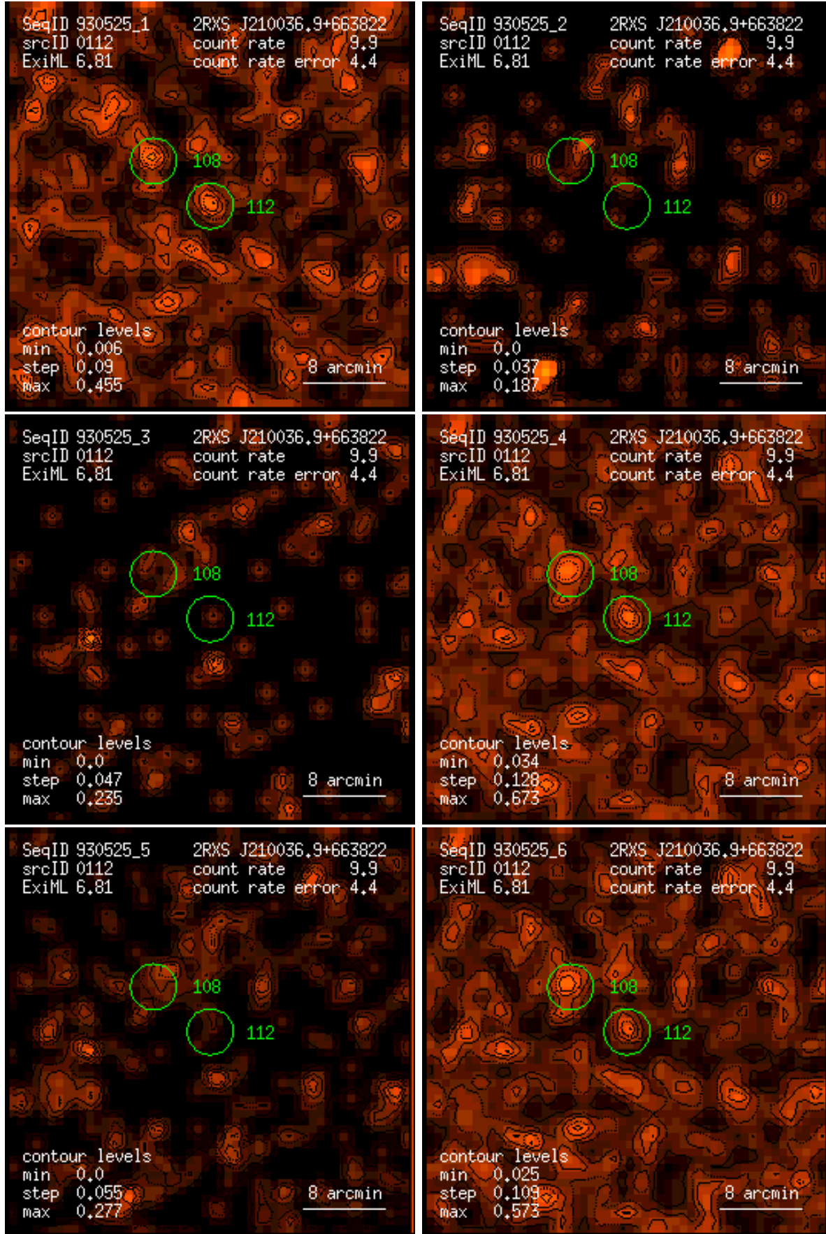
Figure 112: RASS 930525: detection 0112: band rate images, Gaussian filter: (1) PSPC channels 11 – 41, (2) 52 – 90, (3) 91 – 201, (4) 11 – 235, (5) 52 – 201, (6) 11 – 201. Broad band rates in counts/ks. Band rate contour levels in counts/ks/arcmin 2 .
