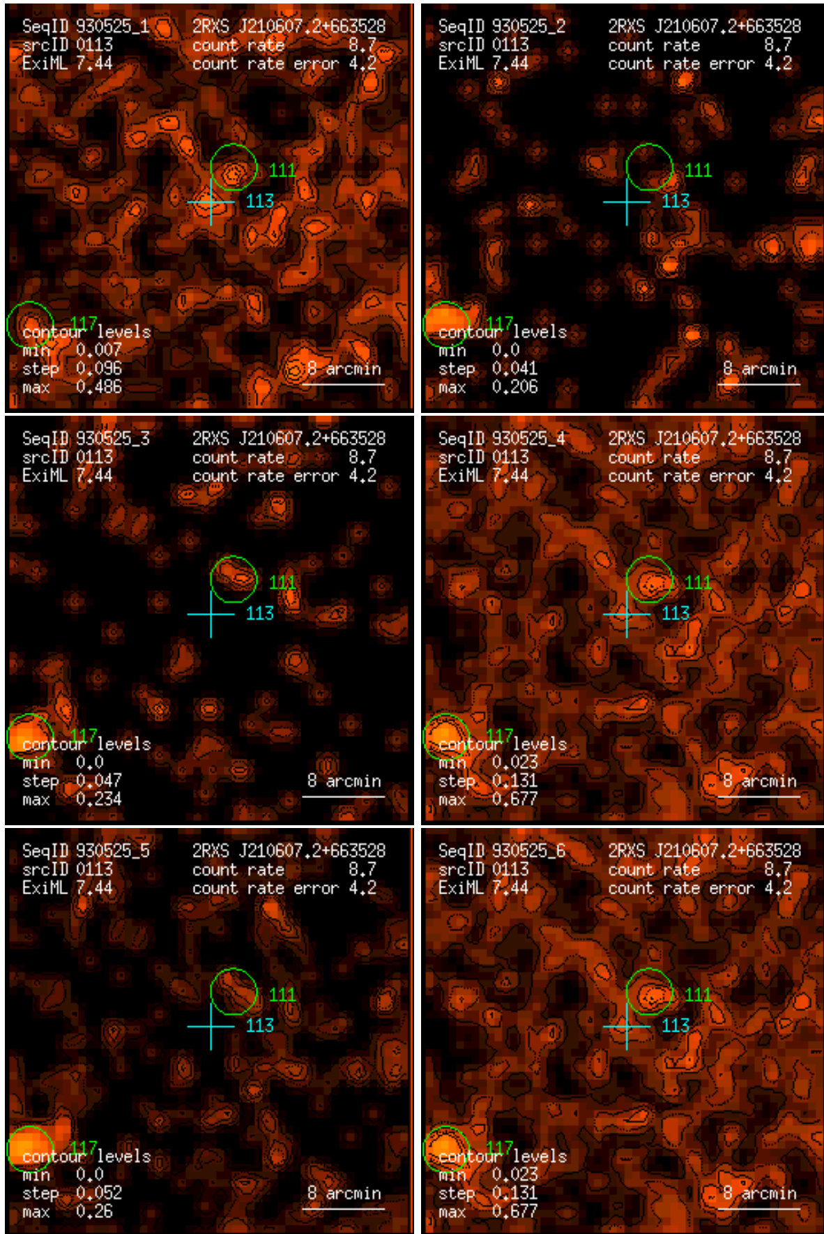
Figure 113: RASS 930525: detection 0113: band rate images, Gaussian filter: (1) PSPC channels 11 – 41, (2) 52 – 90, (3) 91 – 201, (4) 11 – 235, (5) 52 – 201, (6) 11 – 201. Broad band rates in counts/ks. Band rate contour levels in counts/ks/arcmin 2 .
