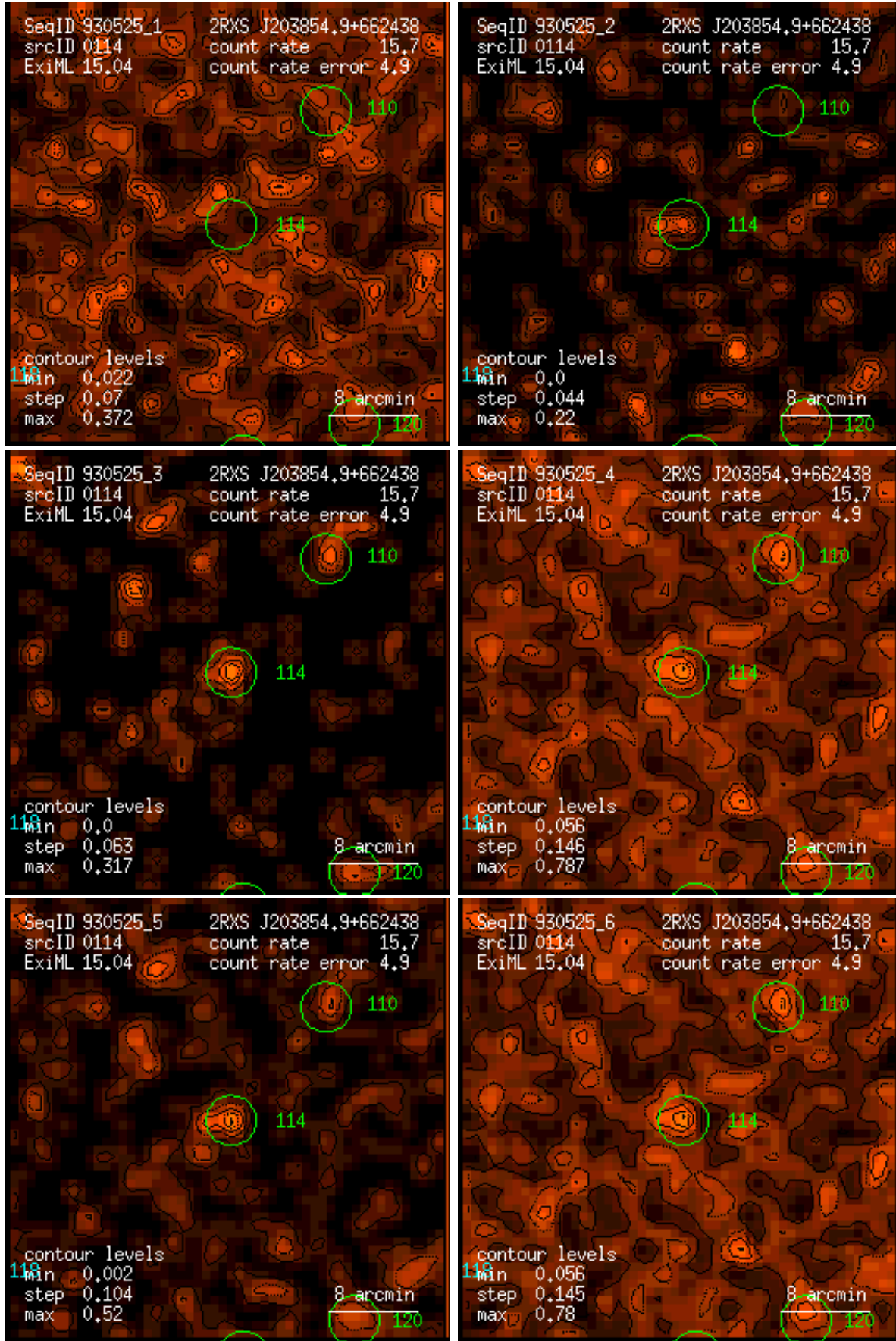
Figure 114: RASS 930525: detection 0114: band rate images, Gaussian filter: (1) PSPC channels 11 – 41, (2) 52 – 90, (3) 91 – 201, (4) 11 – 235, (5) 52 – 201, (6) 11 – 201. Broad band rates in counts/ks. Band rate contour levels in counts/ks/arcmin 2 .
