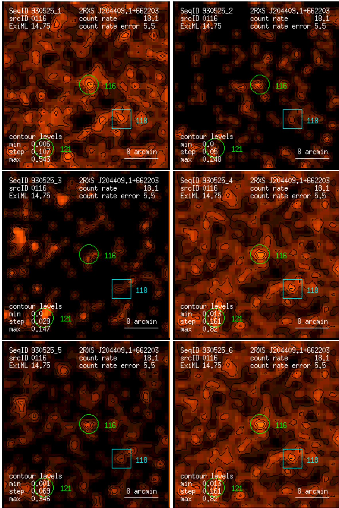
Figure 116: RASS 930525: detection 0116: band rate images, Gaussian filter: (1) PSPC channels 11 – 41, (2) 52 – 90, (3) 91 – 201, (4) 11 – 235, (5) 52 – 201, (6) 11 – 201. Broad band rates in counts/ks. Band rate contour levels in counts/ks/arcmin 2 .
