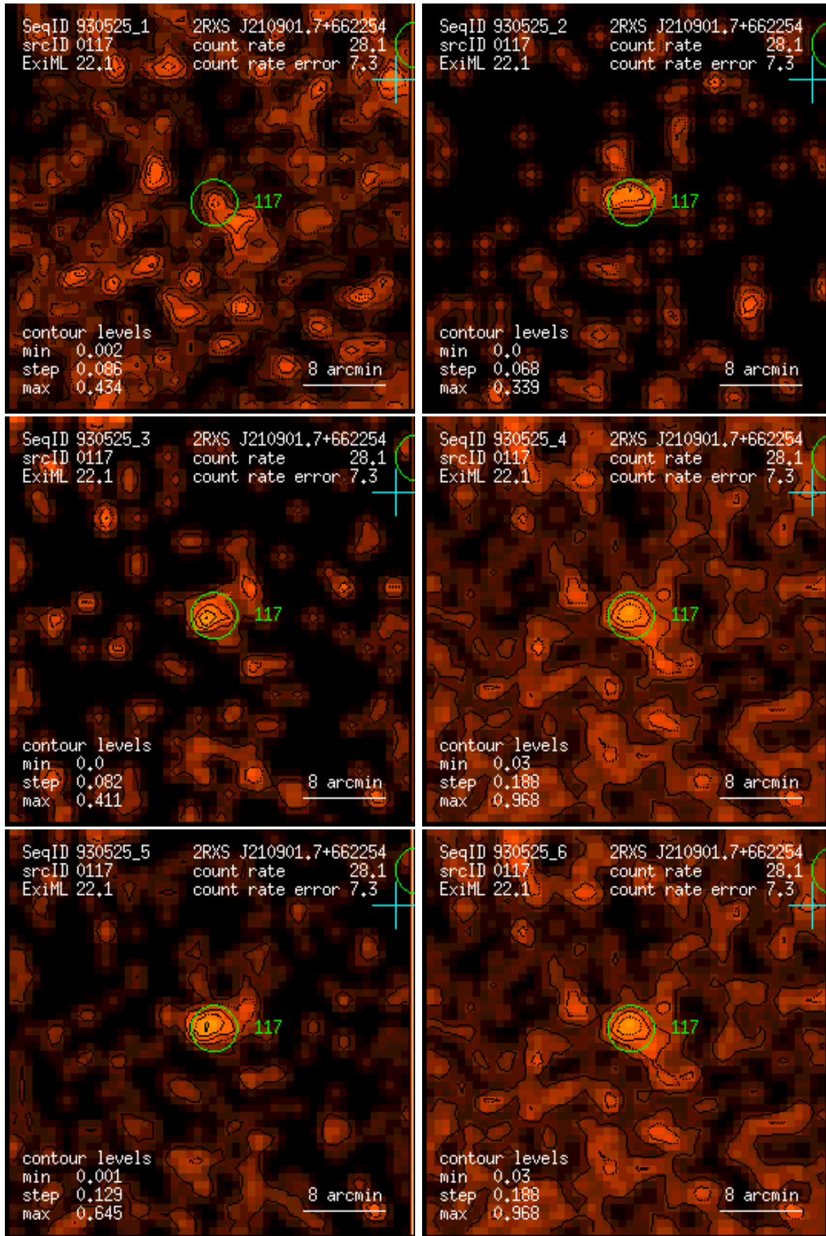
Figure 117: RASS 930525: detection 0117: band rate images, Gaussian filter: (1) PSPC channels 11 – 41, (2) 52 – 90, (3) 91 – 201, (4) 11 – 235, (5) 52 – 201, (6) 11 – 201. Broad band rates in counts/ks. Band rate contour levels in counts/ks/arcmin 2 .
