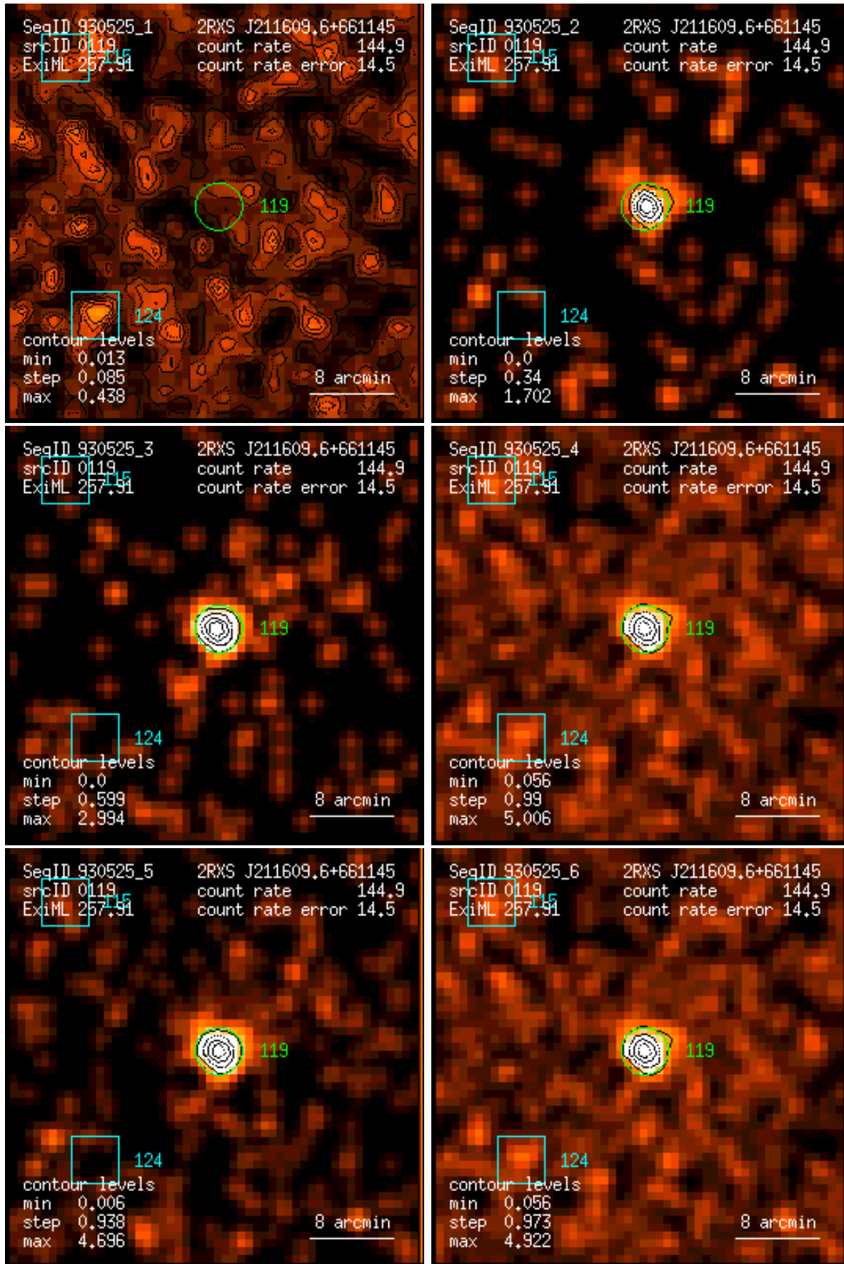
Figure 119: RASS 930525: detection 0119: band rate images, Gaussian filter: (1) PSPC channels 11 – 41, (2) 52 – 90, (3) 91 – 201, (4) 11 – 235, (5) 52 – 201, (6) 11 – 201. Broad band rates in counts/ks. Band rate contour levels in counts/ks/arcmin 2 .
