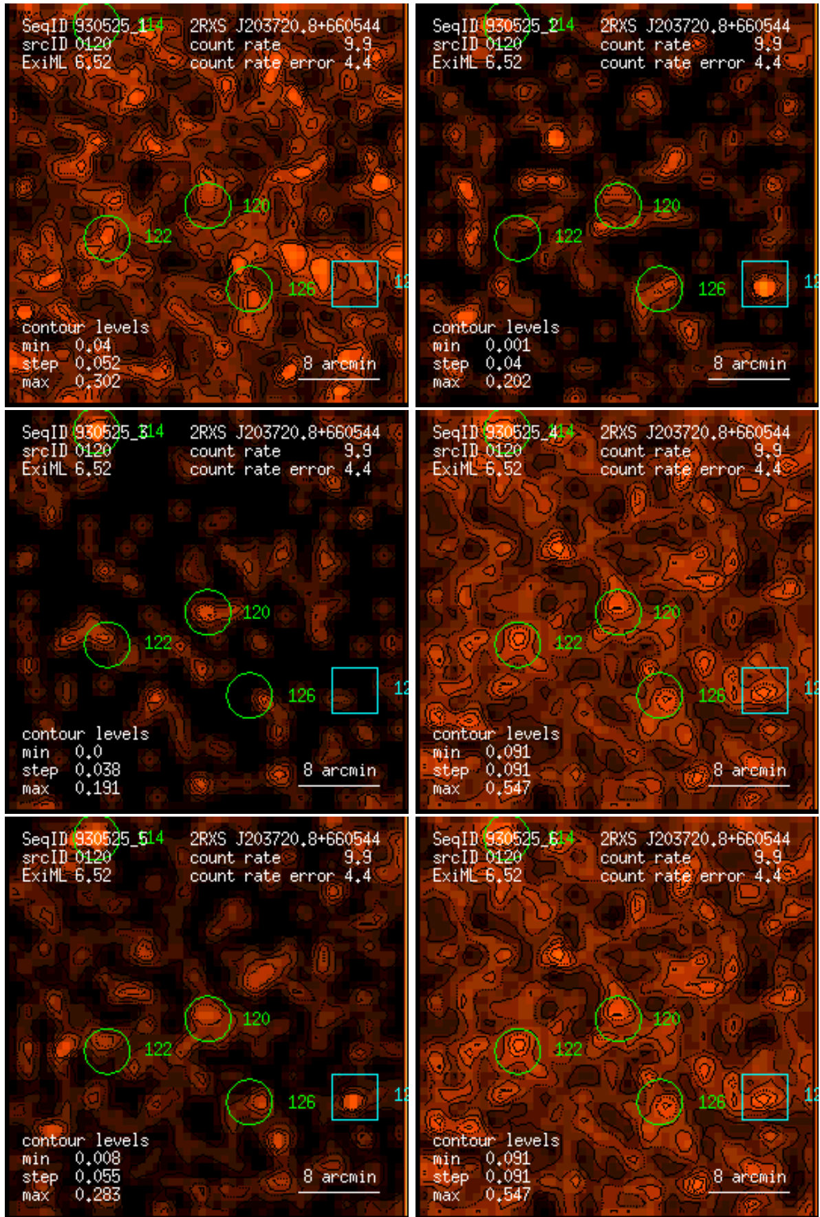
Figure 120: RASS 930525: detection 0120: band rate images, Gaussian filter: (1) PSPC channels 11 – 41, (2) 52 – 90, (3) 91 – 201, (4) 11 – 235, (5) 52 – 201, (6) 11 – 201. Broad band rates in counts/ks. Band rate contour levels in counts/ks/arcmin 2 .
