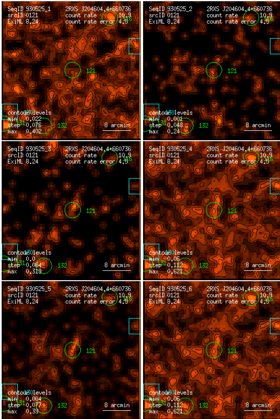
Figure 121: RASS 930525: detection 0121: band rate images, Gaussian filter: (1) PSPC channels 11 – 41, (2) 52 – 90, (3) 91 – 201, (4) 11 – 235, (5) 52 – 201, (6) 11 – 201. Broad band rates in counts/ks. Band rate contour levels in counts/ks/arcmin 2 .
