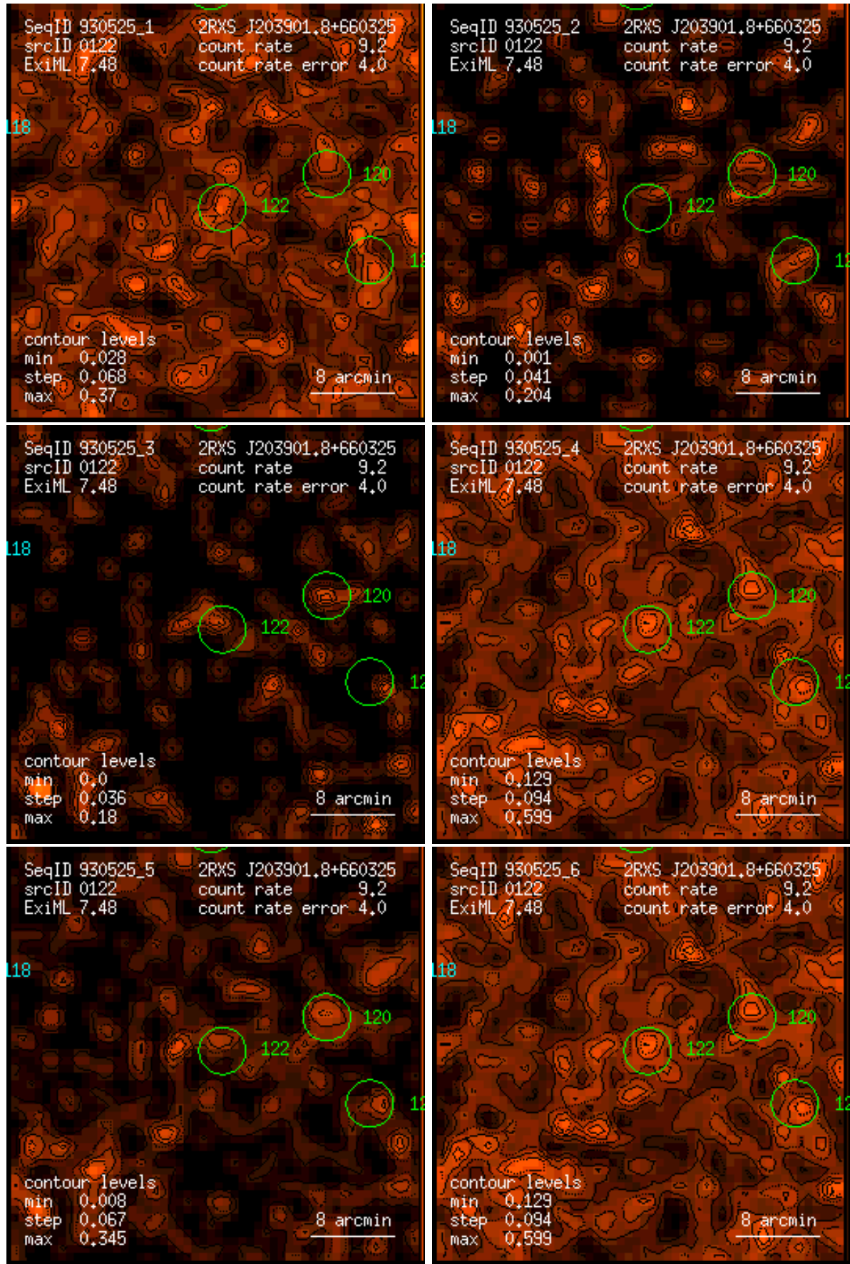
Figure 122: RASS 930525: detection 0122: band rate images, Gaussian filter: (1) PSPC channels 11 – 41, (2) 52 – 90, (3) 91 – 201, (4) 11 – 235, (5) 52 – 201, (6) 11 – 201. Broad band rates in counts/ks. Band rate contour levels in counts/ks/arcmin 2 .
