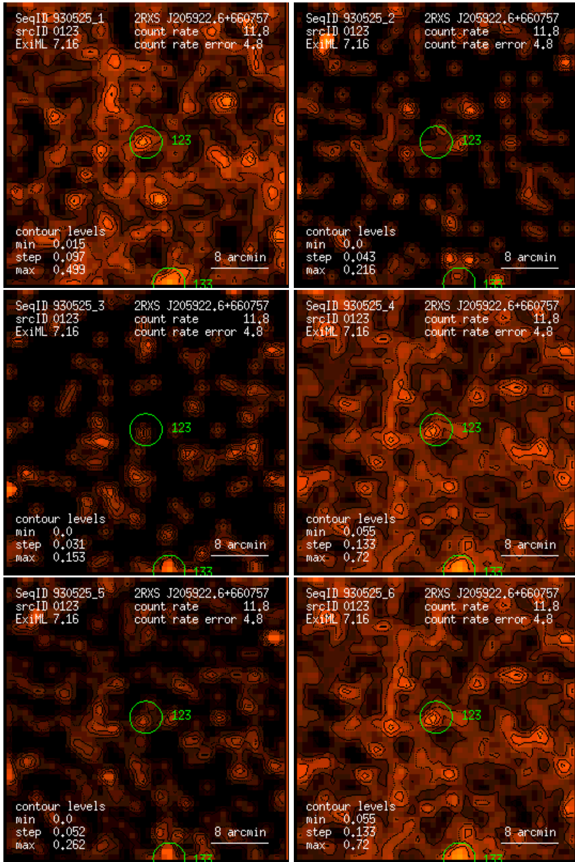
Figure 123: RASS 930525: detection 0123: band rate images, Gaussian filter: (1) PSPC channels 11 – 41, (2) 52 – 90, (3) 91 – 201, (4) 11 – 235, (5) 52 – 201, (6) 11 – 201. Broad band rates in counts/ks. Band rate contour levels in counts/ks/arcmin 2 .
