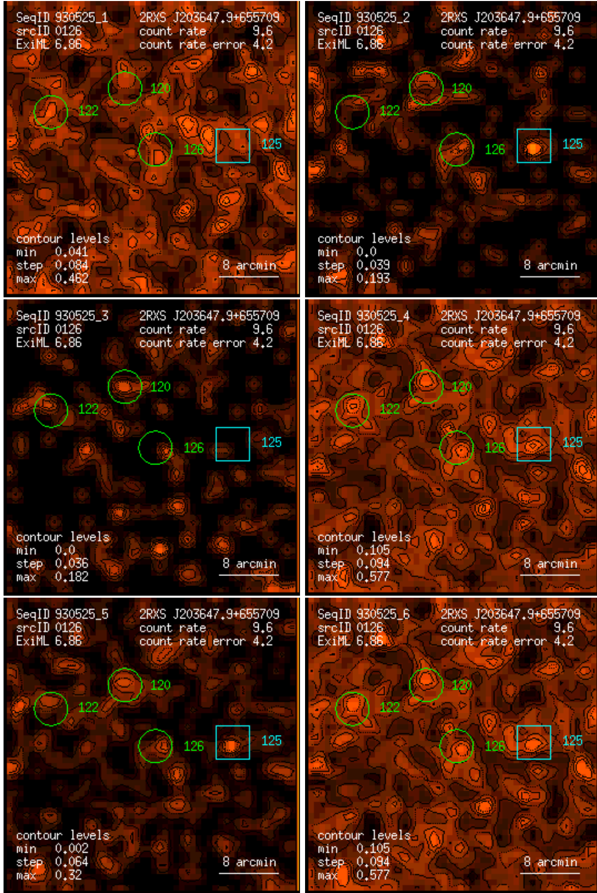
Figure 126: RASS 930525: detection 0126: band rate images, Gaussian filter: (1) PSPC channels 11 – 41, (2) 52 – 90, (3) 91 – 201, (4) 11 – 235, (5) 52 – 201, (6) 11 – 201. Broad band rates in counts/ks. Band rate contour levels in counts/ks/arcmin 2 .
