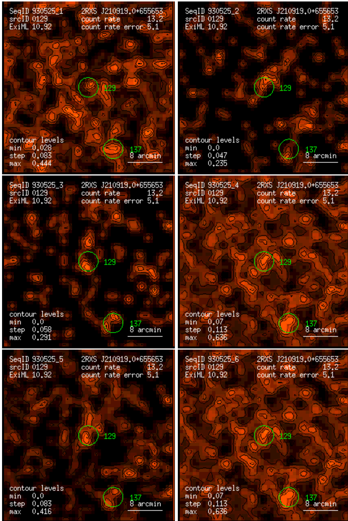
Figure 129: RASS 930525: detection 0129: band rate images, Gaussian filter: (1) PSPC channels 11 – 41, (2) 52 – 90, (3) 91 – 201, (4) 11 – 235, (5) 52 – 201, (6) 11 – 201. Broad band rates in counts/ks. Band rate contour levels in counts/ks/arcmin 2 .
