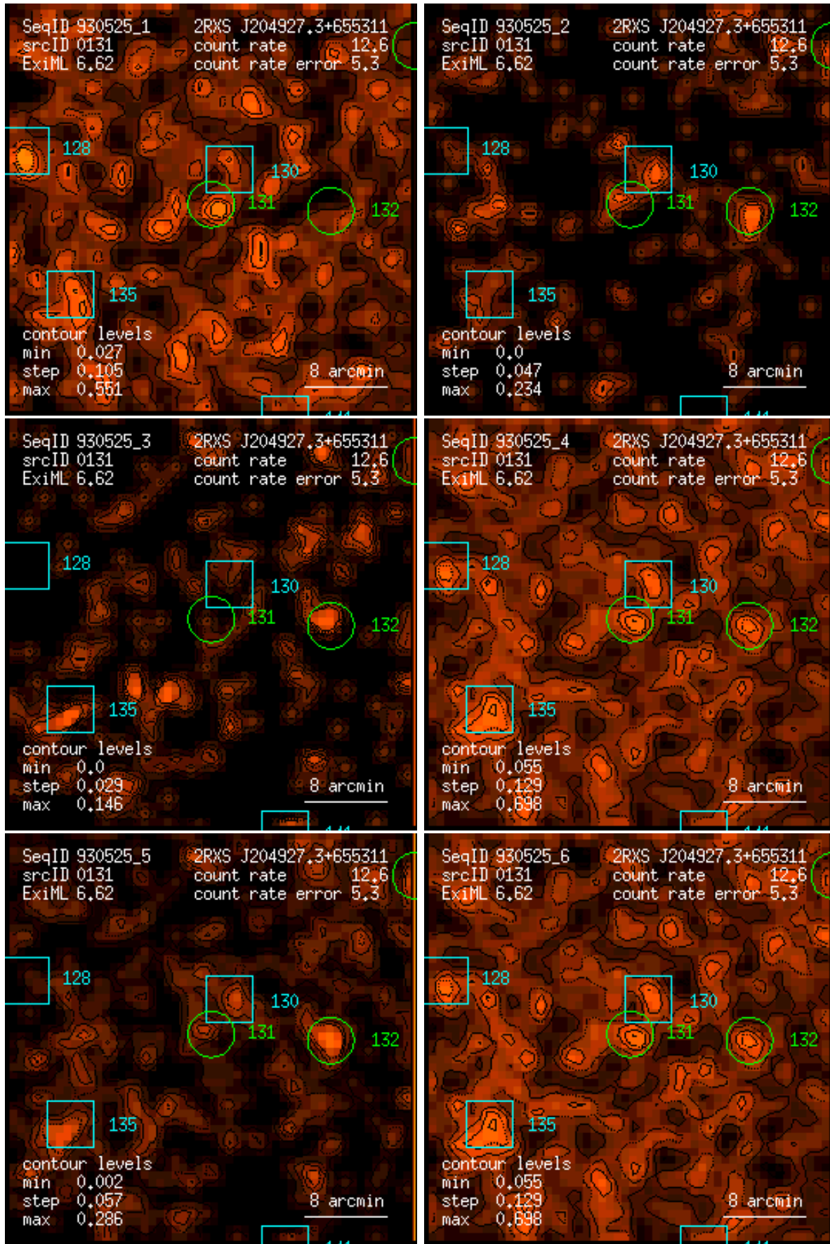
Figure 131: RASS 930525: detection 0131: band rate images, Gaussian filter: (1) PSPPC channels 11 – 41, (2) 52 – 90, (3) 91 – 201, (4) 11 – 235, (5) 52 – 201, (6) 11 – 201. Broad band rates in counts/ks. Band rate contour levels in counts/ks/arcmin 2 .
