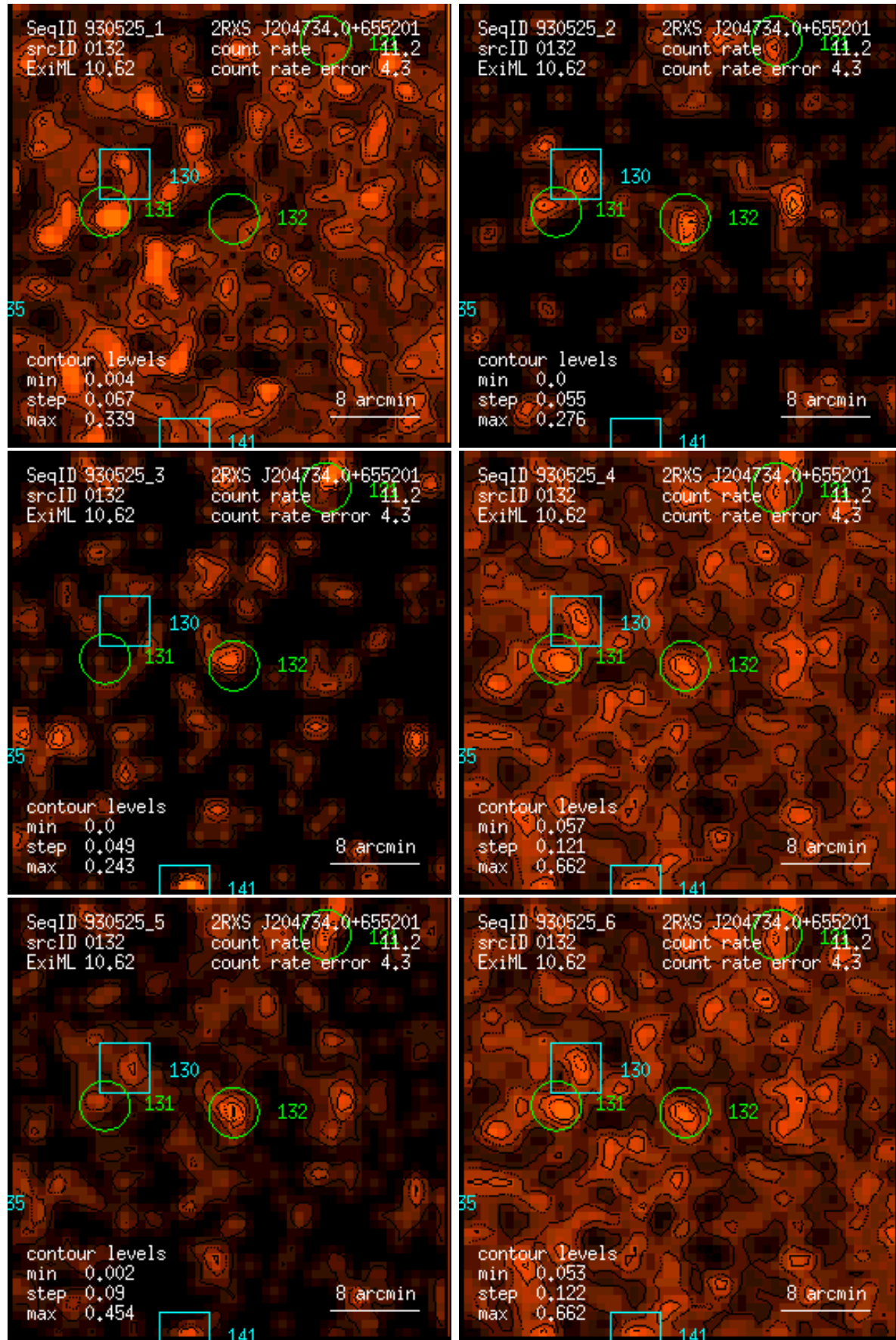
Figure 132: RASS 930525: detection 0132: band rate images, Gaussian filter: (1) PSPC channels 11 – 41, (2) 52 – 90, (3) 91 – 201, (4) 11 – 235, (5) 52 – 201, (6) 11 – 201. Broad band rates in counts/ks. Band rate contour levels in counts/ks/arcmin 2 .
