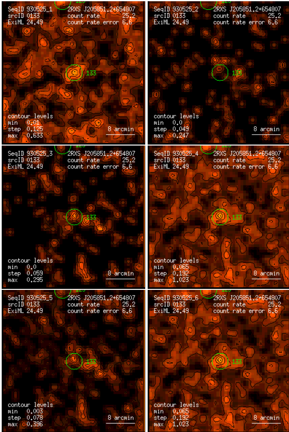
Figure 133: RASS 930525: detection 0133: band rate images, Gaussian filter: (1) PSPC channels 11 – 41, (2) 52 – 90, (3) 91 – 201, (4) 11 – 235, (5) 52 – 201, (6) 11 – 201. Broad band rates in counts/ks. Band rate contour levels in counts/ks/arcmin 2 .
