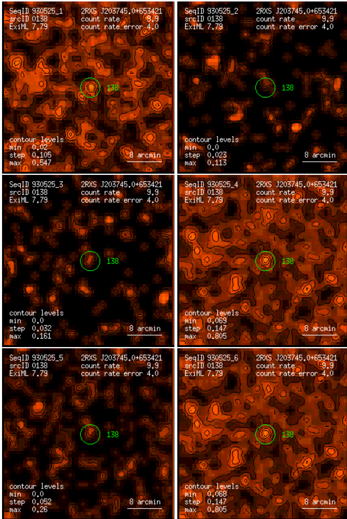
Figure 138: RASS 930525: detection 0138: band rate images, Gaussian filter: (1) PSPC channels 11 – 41, (2) 52 – 90, (3) 91 – 201, (4) 11 – 235, (5) 52 – 201, (6) 11 – 201. Broad band rates in counts/ks. Band rate contour levels in counts/ks/arcmin 2 .
