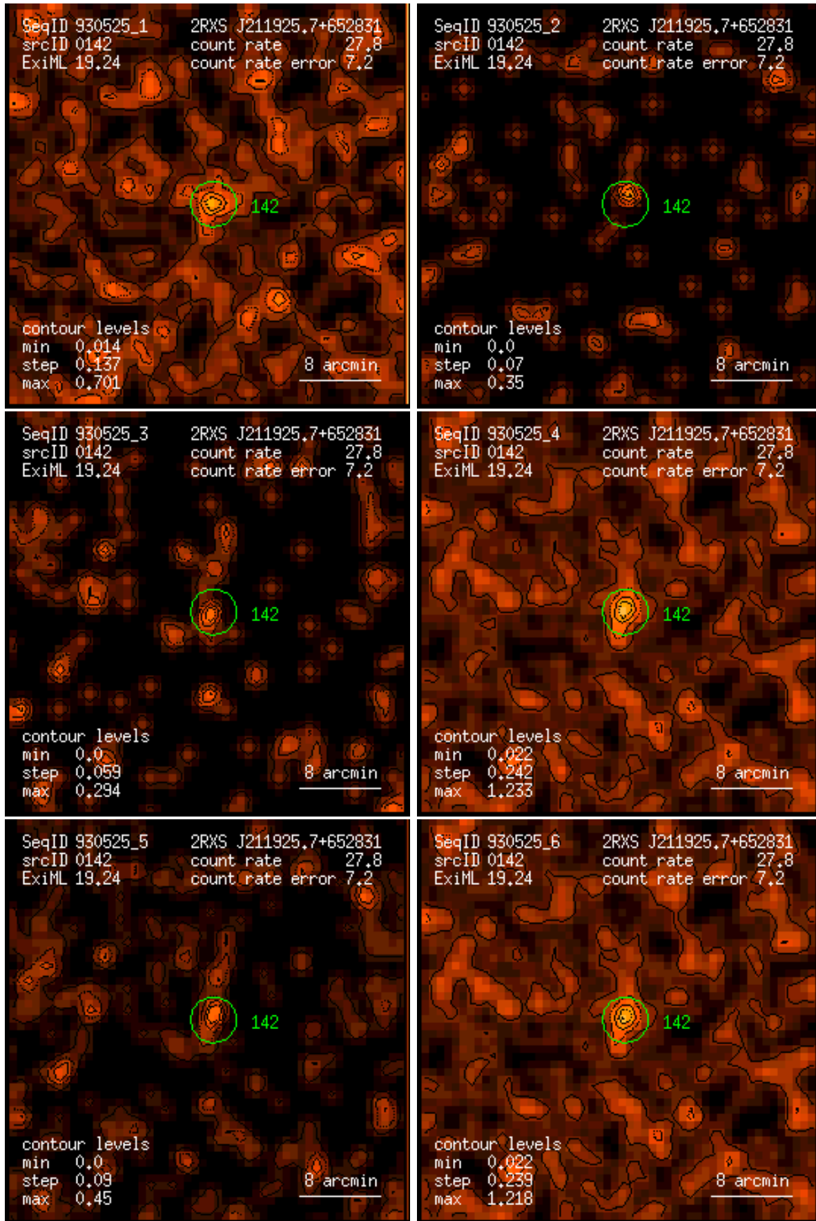
Figure 142: RASS 930525: detection 0142: band rate images, Gaussian filter: (1) PSPC channels 11 – 41, (2) 52 – 90, (3) 91 – 201, (4) 11 – 235, (5) 52 – 201, (6) 11 – 201. Broad band rates in counts/ks. Band rate contour levels in counts/ks/arcmin 2 .
