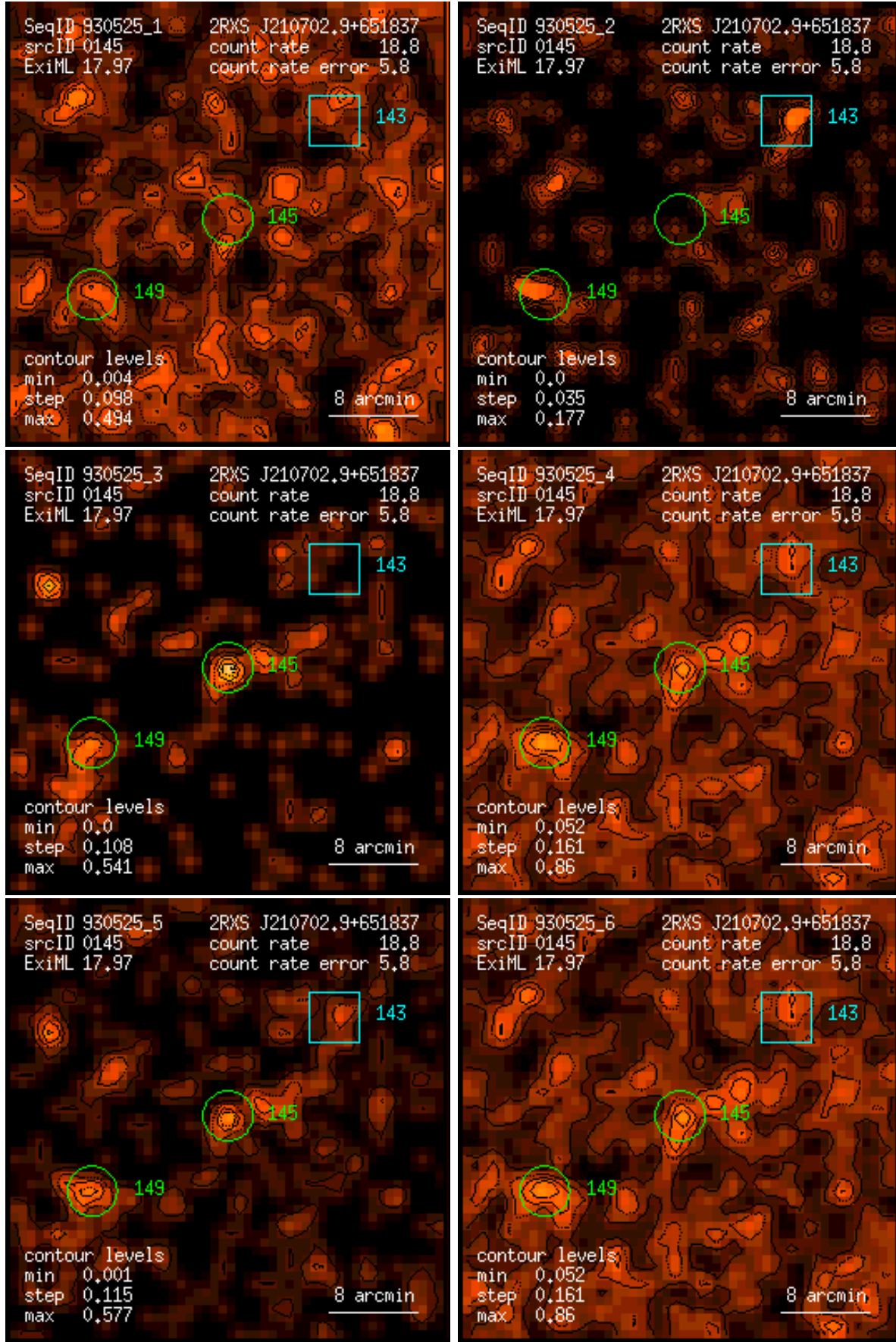
Figure 145: RASS 930525: detection 0145: band rate images, Gaussian filter: (1) PSPC channels 11 – 41, (2) 52 – 90, (3) 91 – 201, (4) 11 – 235, (5) 52 – 201, (6) 11 – 201. Broad band rates in counts/ks. Band rate contour levels in counts/ks/arcmin 2 .
