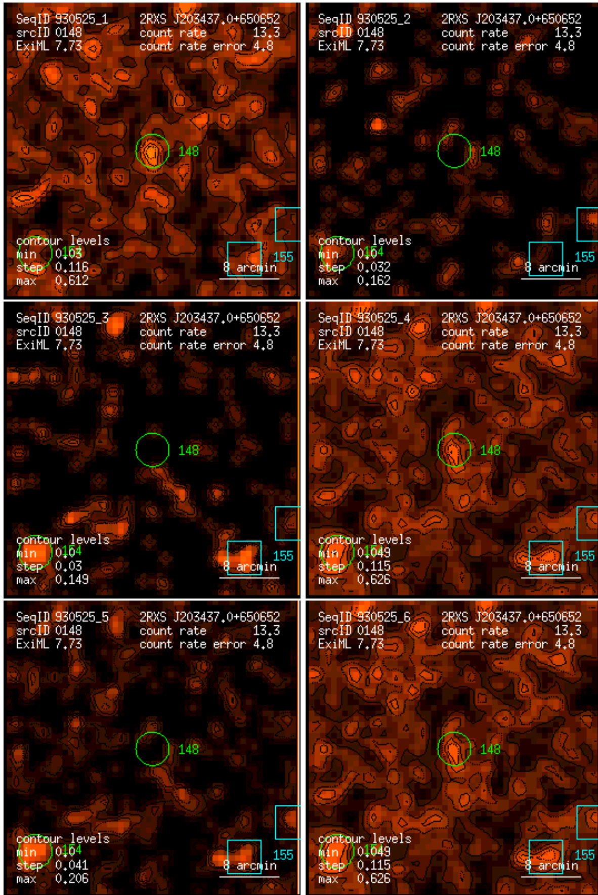
Figure 148: RASS 930525: detection 0148: band rate images, Gaussian filter: (1) PSPC channels 11 – 41, (2) 52 – 90, (3) 91 – 201, (4) 11 – 235, (5) 52 – 201, (6) 11 – 201. Broad band rates in counts/ks. Band rate contour levels in counts/ks/arcmin 2 .
