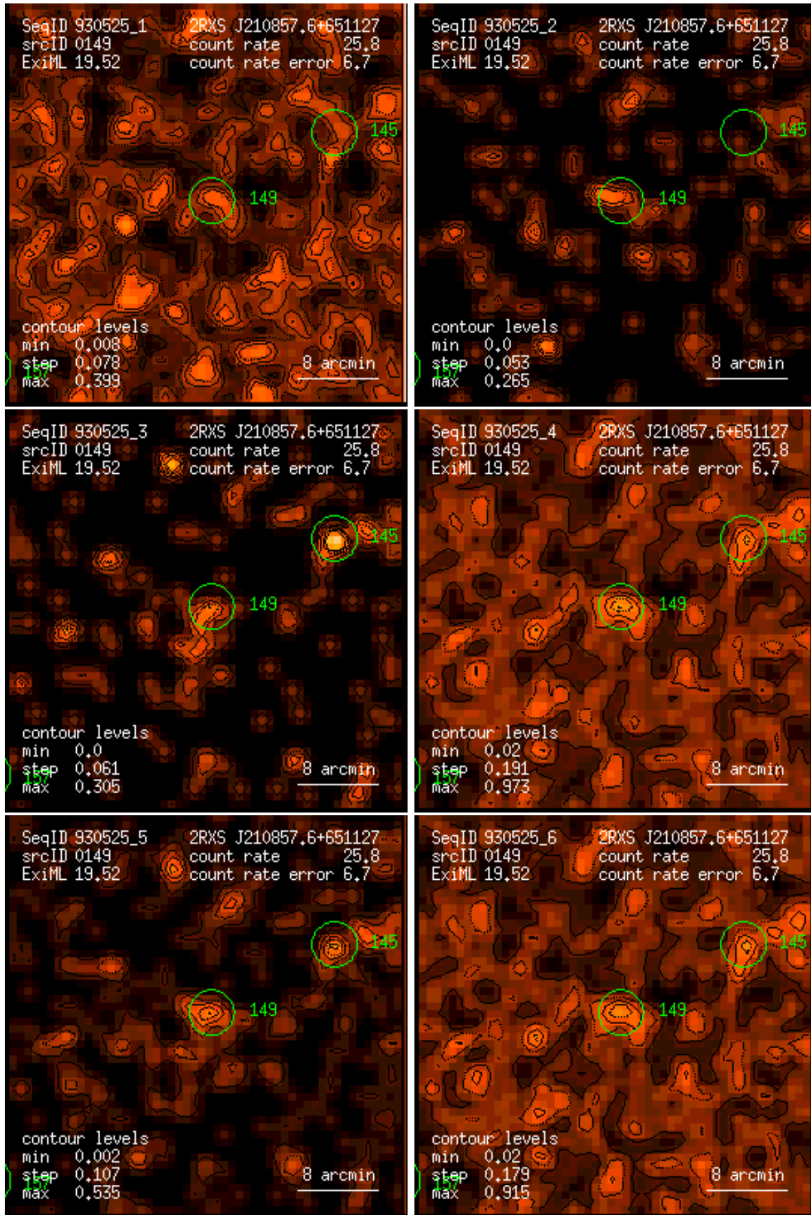
Figure 149: RASS 930525: detection 0149: band rate images, Gaussian filter: (1) PSPC channels 11 – 41, (2) 52 – 90, (3) 91 – 201, (4) 11 – 235, (5) 52 – 201, (6) 11 – 201. Broad band rates in counts/ks. Band rate contour levels in counts/ks/arcmin 2 .
