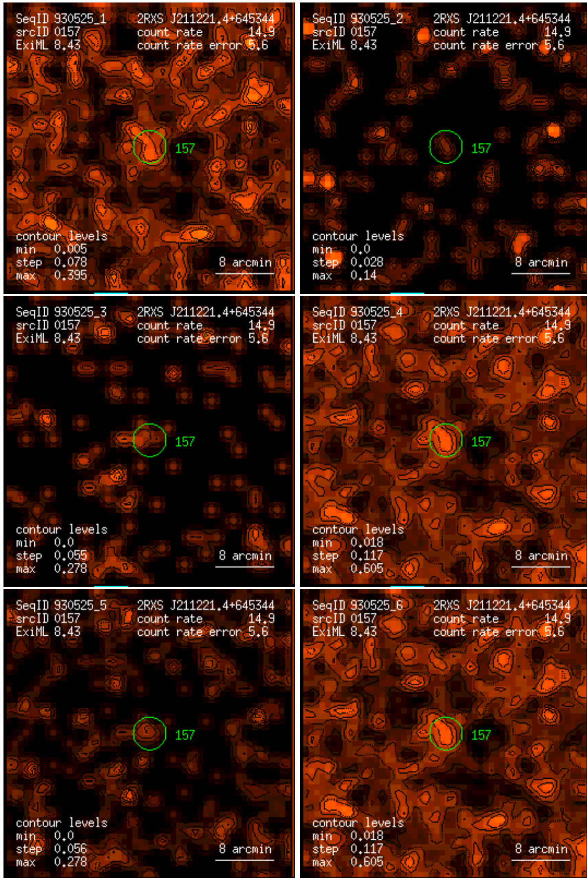
Figure 157: RASS 930525: detection 0157: band rate images, Gaussian filter: (1) PSPC channels 11 – 41, (2) 52 – 90, (3) 91 – 201, (4) 11 – 235, (5) 52 – 201, (6) 11 – 201. Broad band rates in counts/ks. Band rate contour levels in counts/ks/arcmin 2 .
